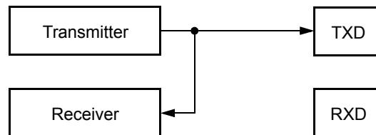
Figure 16-31. Loop Operation (LOOPS = 1, RSRC = 0)
