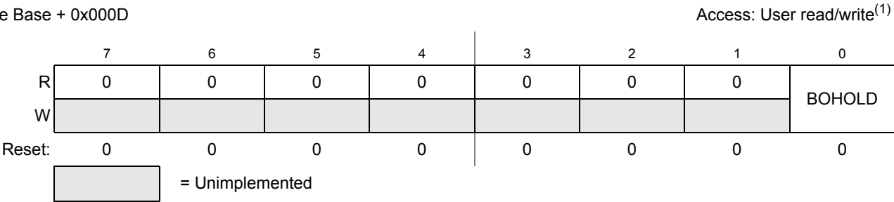
Figure 13-17. MSCAN Miscellaneous Register (CANMISC)
