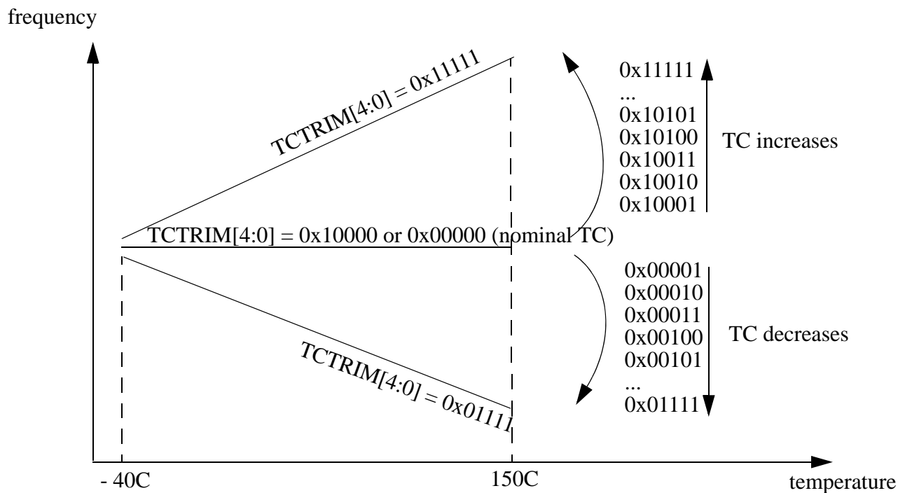
Figure 8-34. Influence of TCTRIM[4:0] on the Temperature Coefficient
