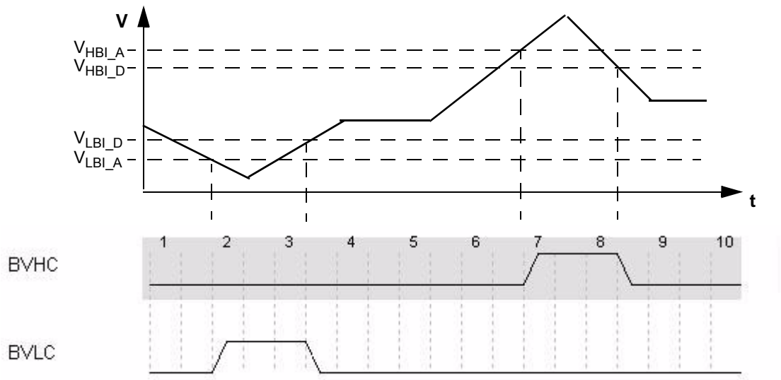
Figure 10-5. BATS Voltage Sensing
