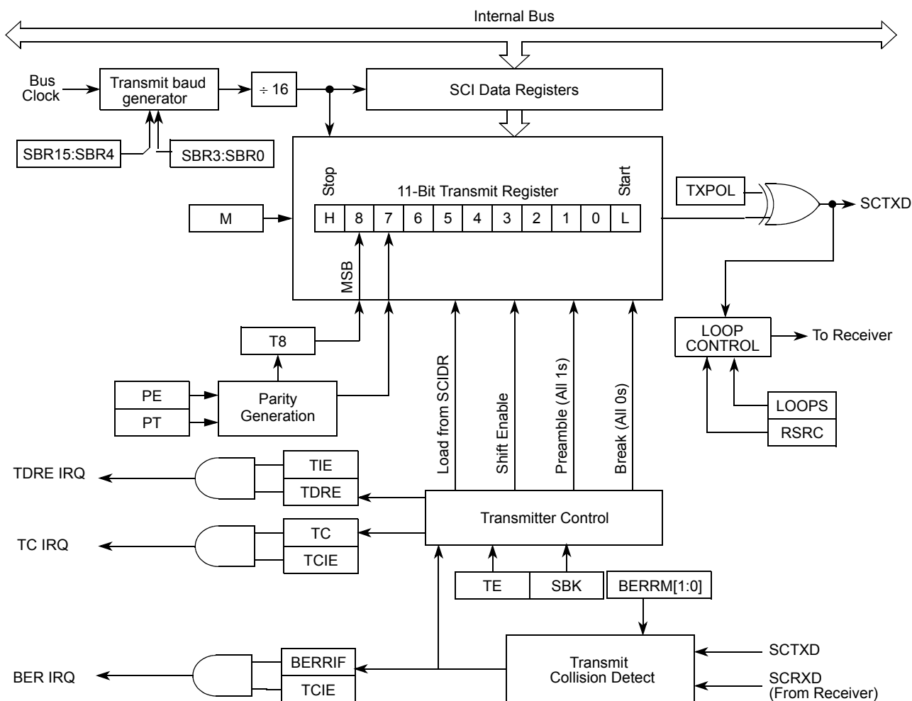
Figure 16-16. Transmitter Block Diagram
