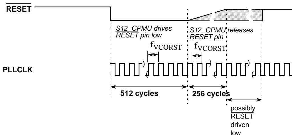
Figure 8-45. RESET Timing
