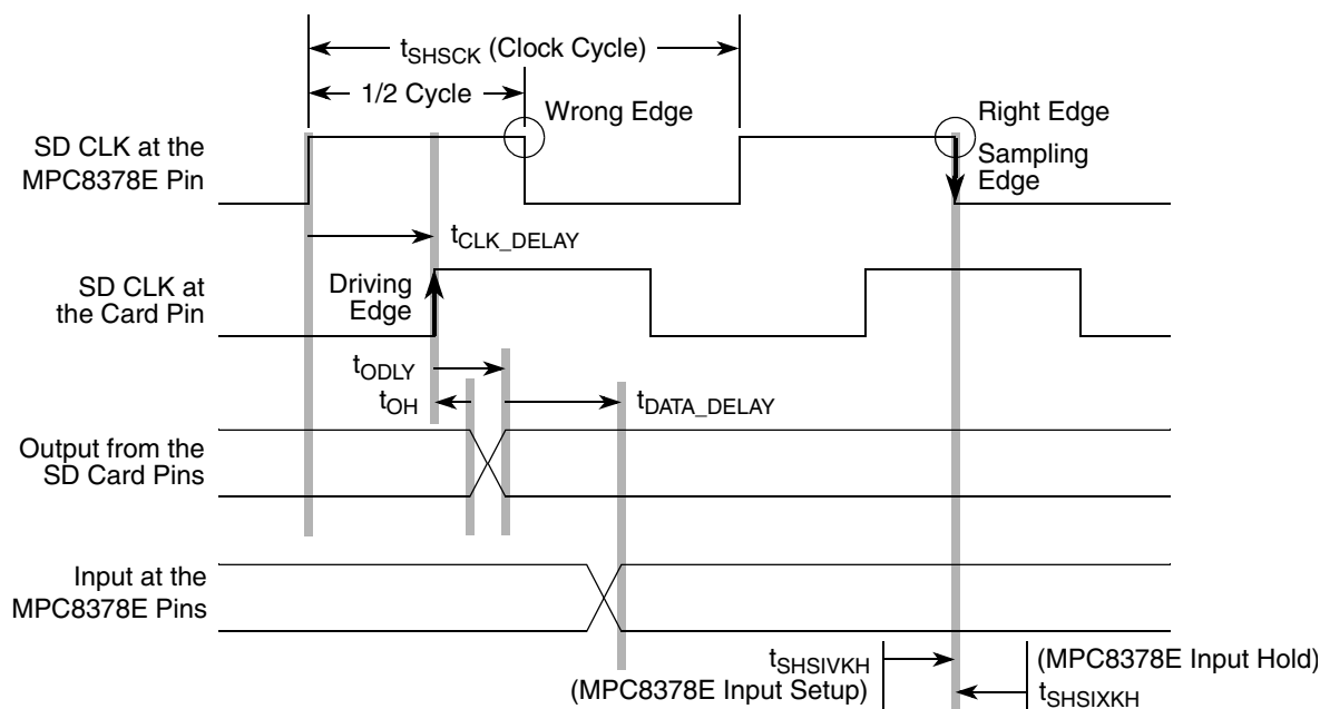
Figure 35. High-Speed Input Path
