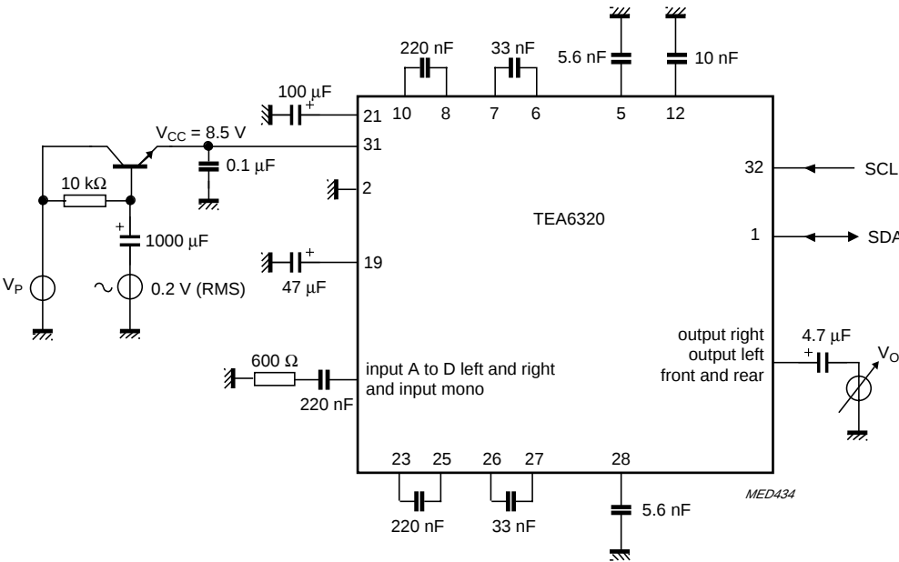
Fig.14 Test circuit for power supply ripple rejection (RR).
