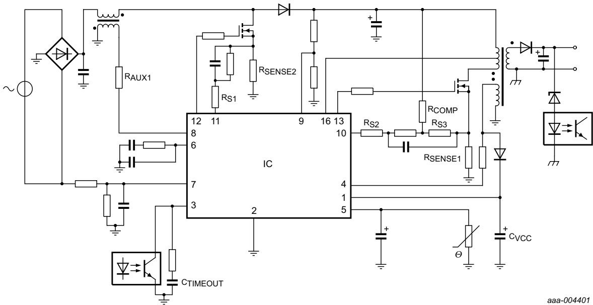
Fig 17. Typical application diagram for the TEA1752T IC
