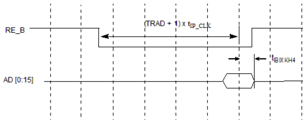
Figure 56. t_{IBIXKH4} Timings
