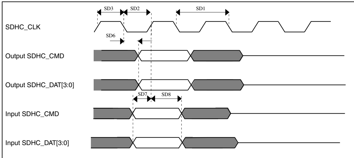
Figure 29. SDHC timing
