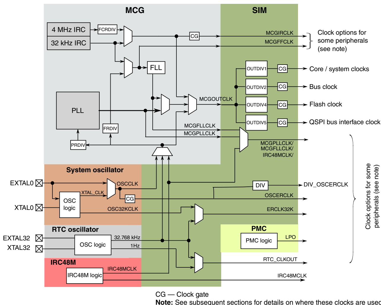
Figure 3. Clocking diagram
