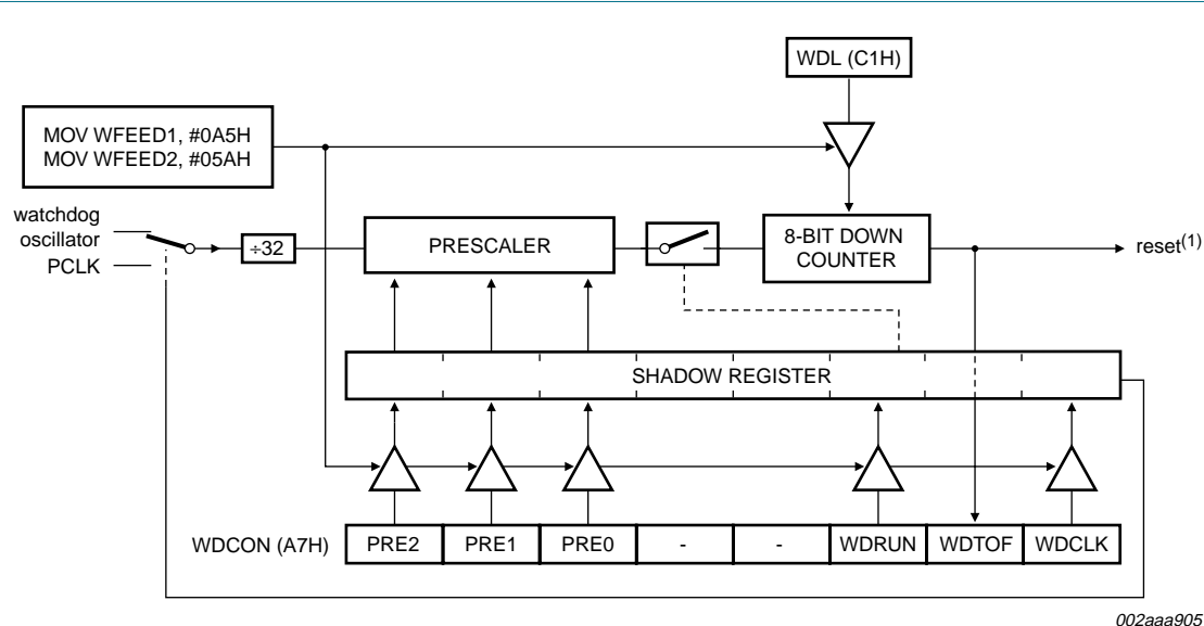
Fig 23. Watchdog timer in Watchdog mode (WDTE = '1')
