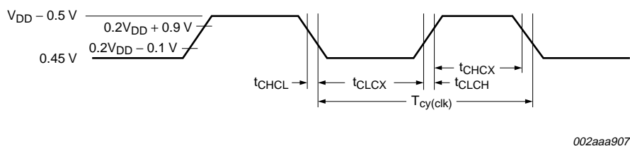
Fig 25. External clock timing
