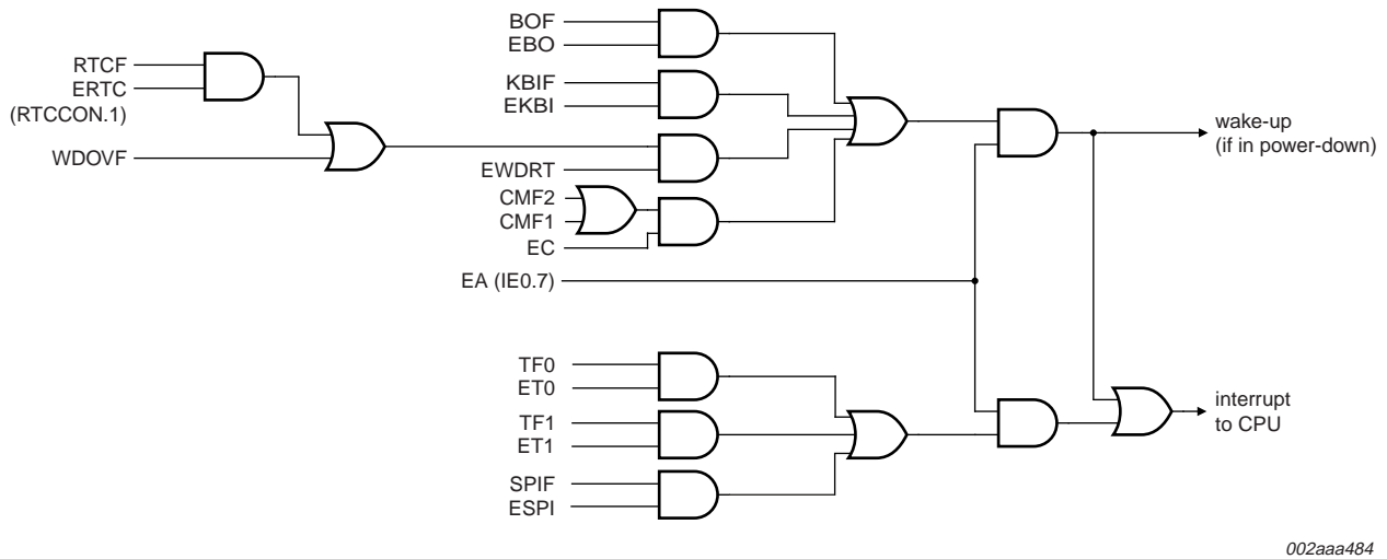
Fig 13. Interrupt sources, interrupt enables, and power-down wake-up sources (P89LPC912)
