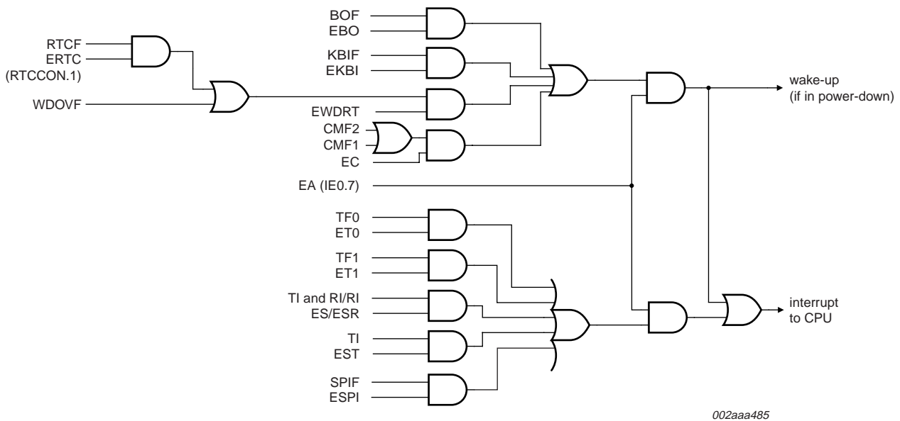
Fig 14. Interrupt sources, interrupt enables, and power-down wake-up sources (P89LPC913, P89LPC914)
