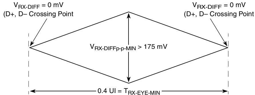
Figure 70. Minimum Receiver Eye Timing and Voltage Compliance Specification
