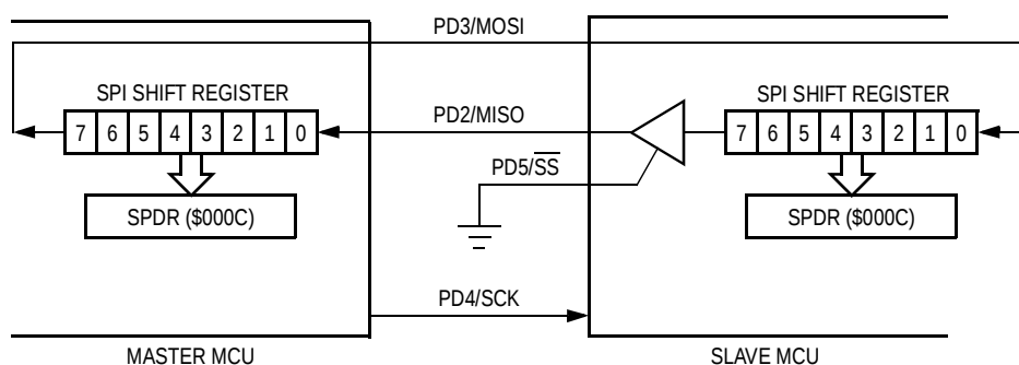
Figure 11-3. Master/Slave Connections
