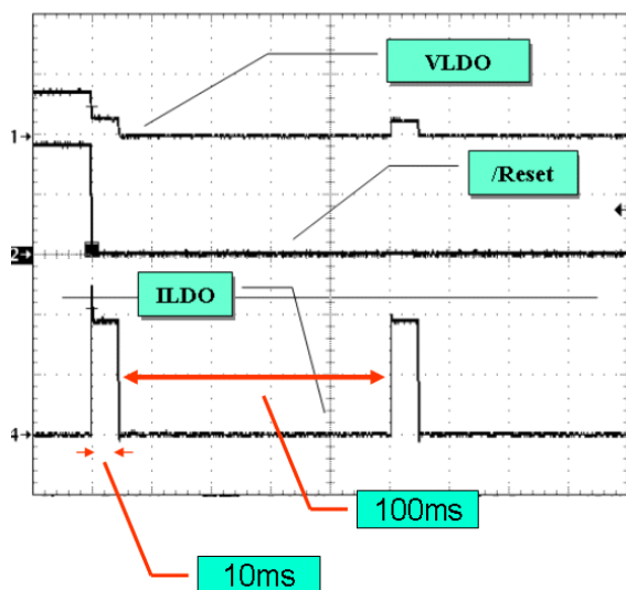
Figure 15. LDO Converter Over-current Protection
