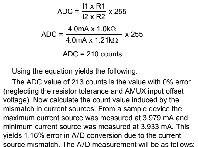
\text{ADC} = \frac{3.933 \text{ mA} \times 1.0\text{k}\Omega}{3.979 \text{ mA} \times 1.21\text{k}\Omega} \times 255 \text{ADC} = 208 \text{ counts} This A/D conversion is 1.16% low in value. The error correction factor of 1.0115 may be used to correct the value: \text{ADC} = 208 \text{ counts} \times 1.0116 \text{ADC} = 210 \text{ counts} An error correction factor may then be stored in E 2 memory and used in the A/D calculation for the specific input. Each input used as analog measurement will have a dedicated calibrated error correction factor.
