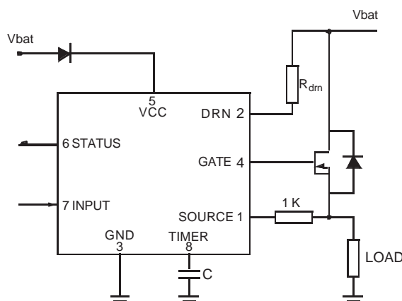
Figure 18. 33198 Reverse Battery
