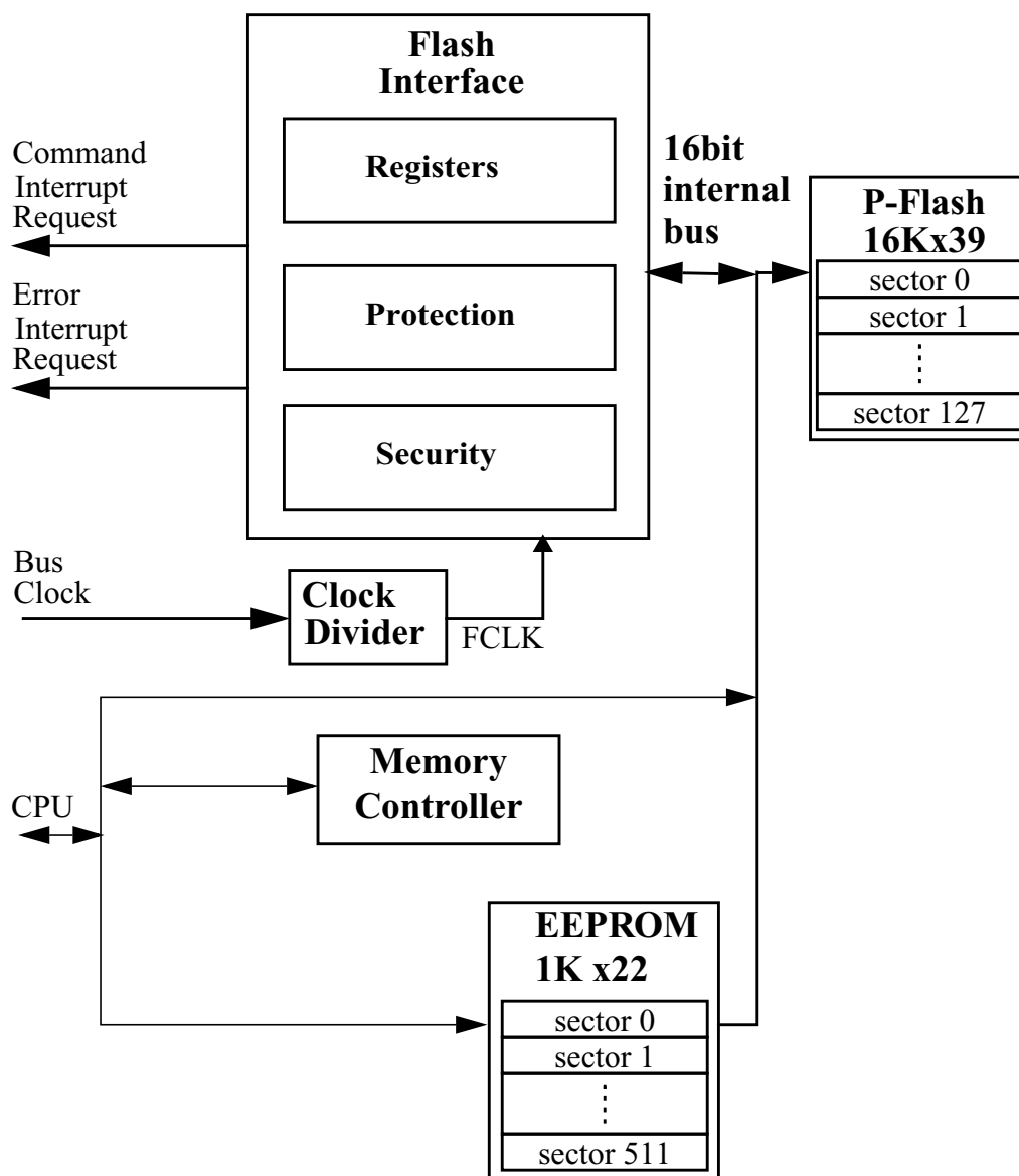
Figure 21-1. FTMZ64K2K Block Diagram
