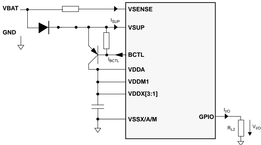
Figure A-2. Supply Currents Overview
