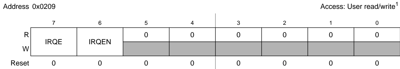
Figure 2-5. IRQ Control Register (IRQCR)
