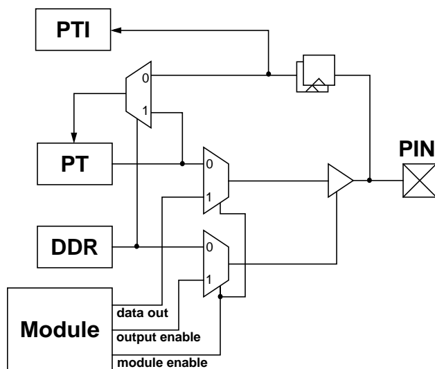
Figure 2-22. Illustration of I/O pin functionality
