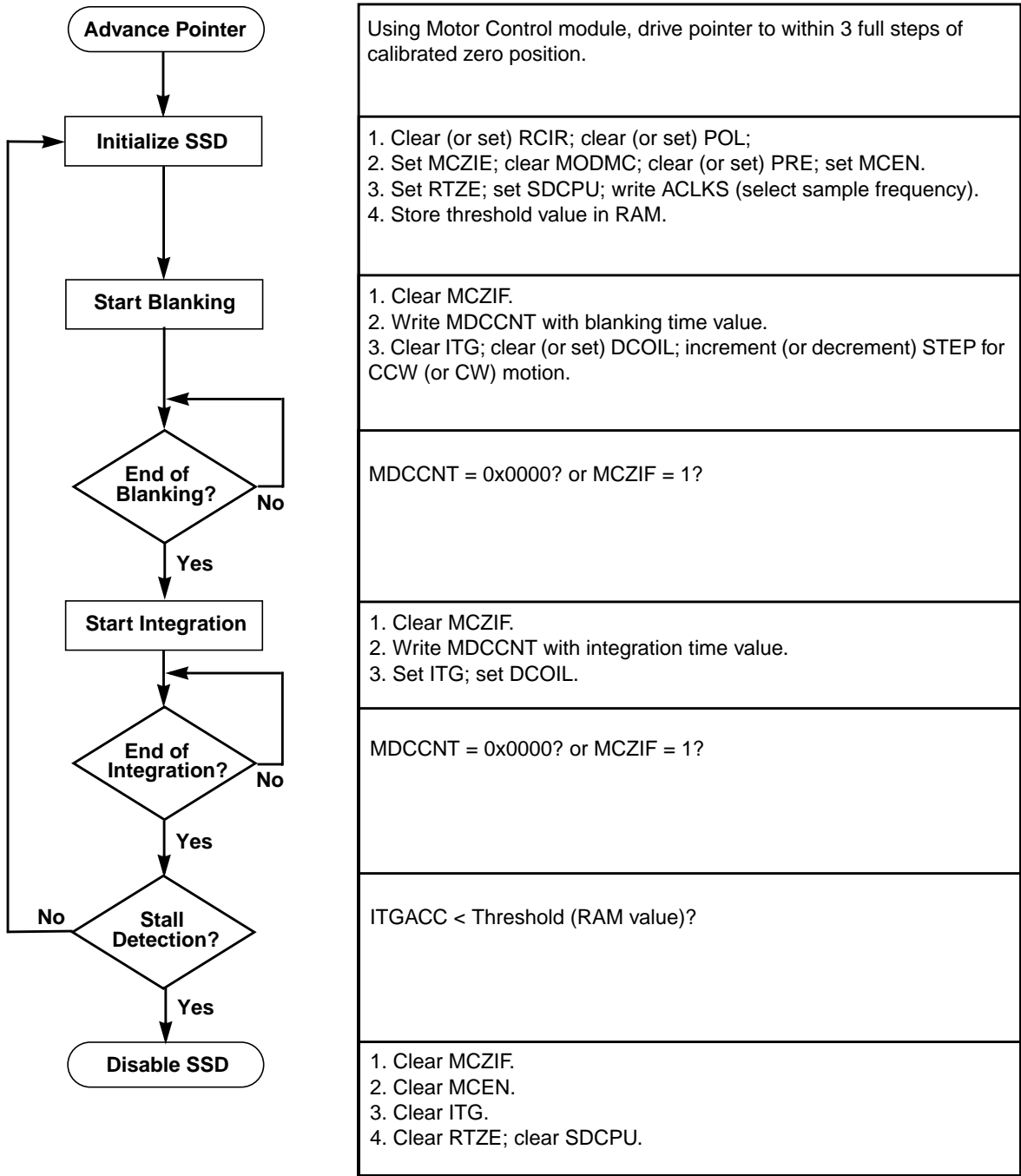
Figure 17-15. Return-to-Zero Flowchart
