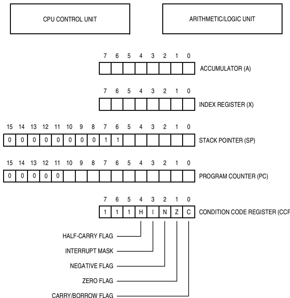
Figure 3-1. Programming Model
