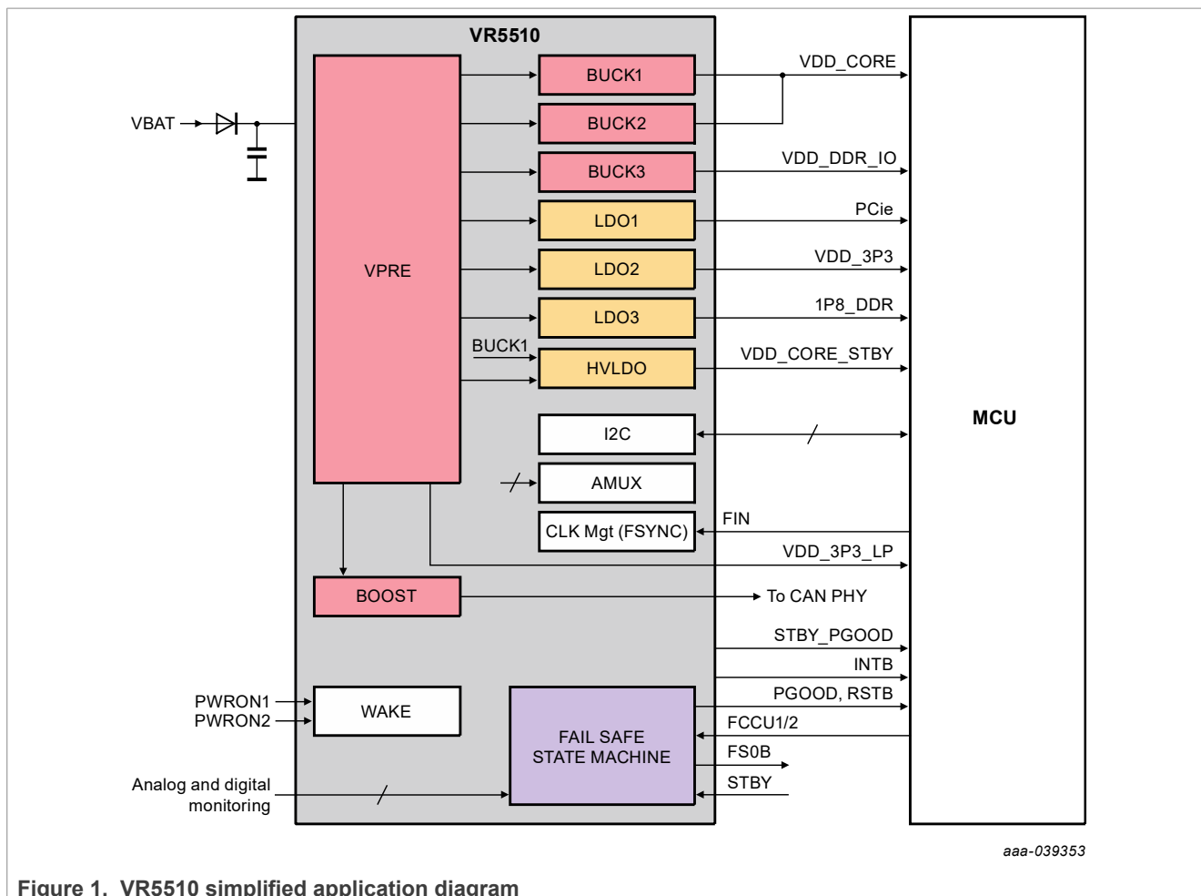
Figure 1. VR5510 simplified application diagram
