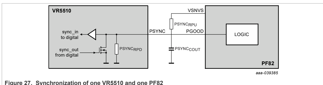
Figure 27. Synchronization of one VR5510 and one PF82
