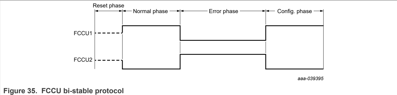
Figure 35. FCCU bi-stable protocol
