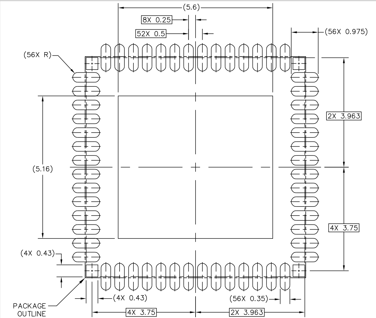
PCB DESIGN GUIDELINES – SOLDER MASK OPENING PATTERN
