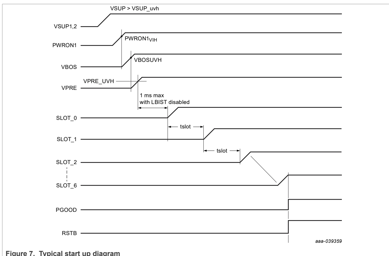
Figure 7. Typical start up diagram
