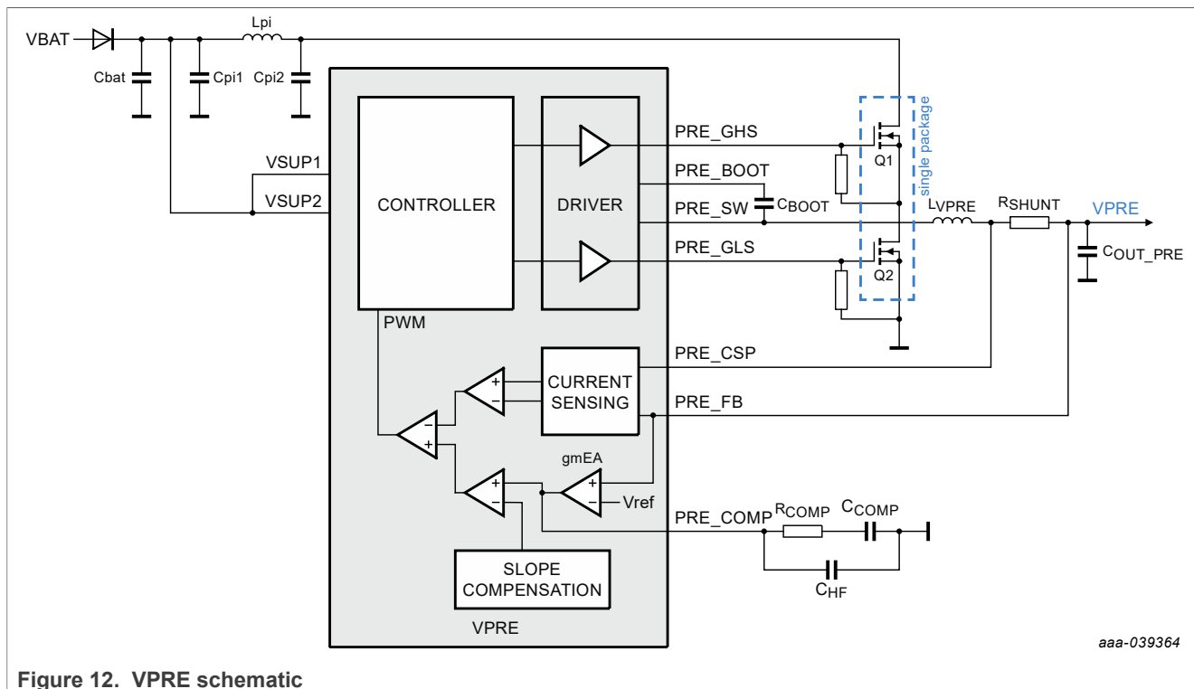
Figure 12. VPRE schematic
