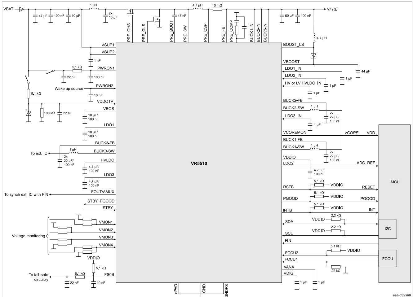
Figure 28. Application schematic
