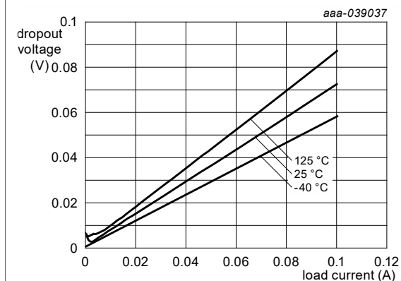
Figure 33. Dropout voltage – LDO1, LDO3: V_{SD} - V_{OUT} = 3.3\text{ V}
