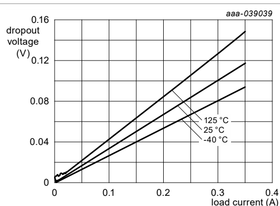
Figure 32. Dropout voltage – LDO4: V33 - V_{OUT} = 3.3\text{ V}
