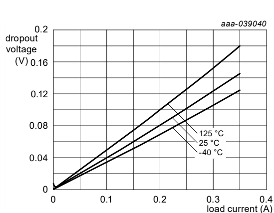
Figure 34. Dropout voltage: LDO4 - V_{OUT} = 1.8\text{ V}
