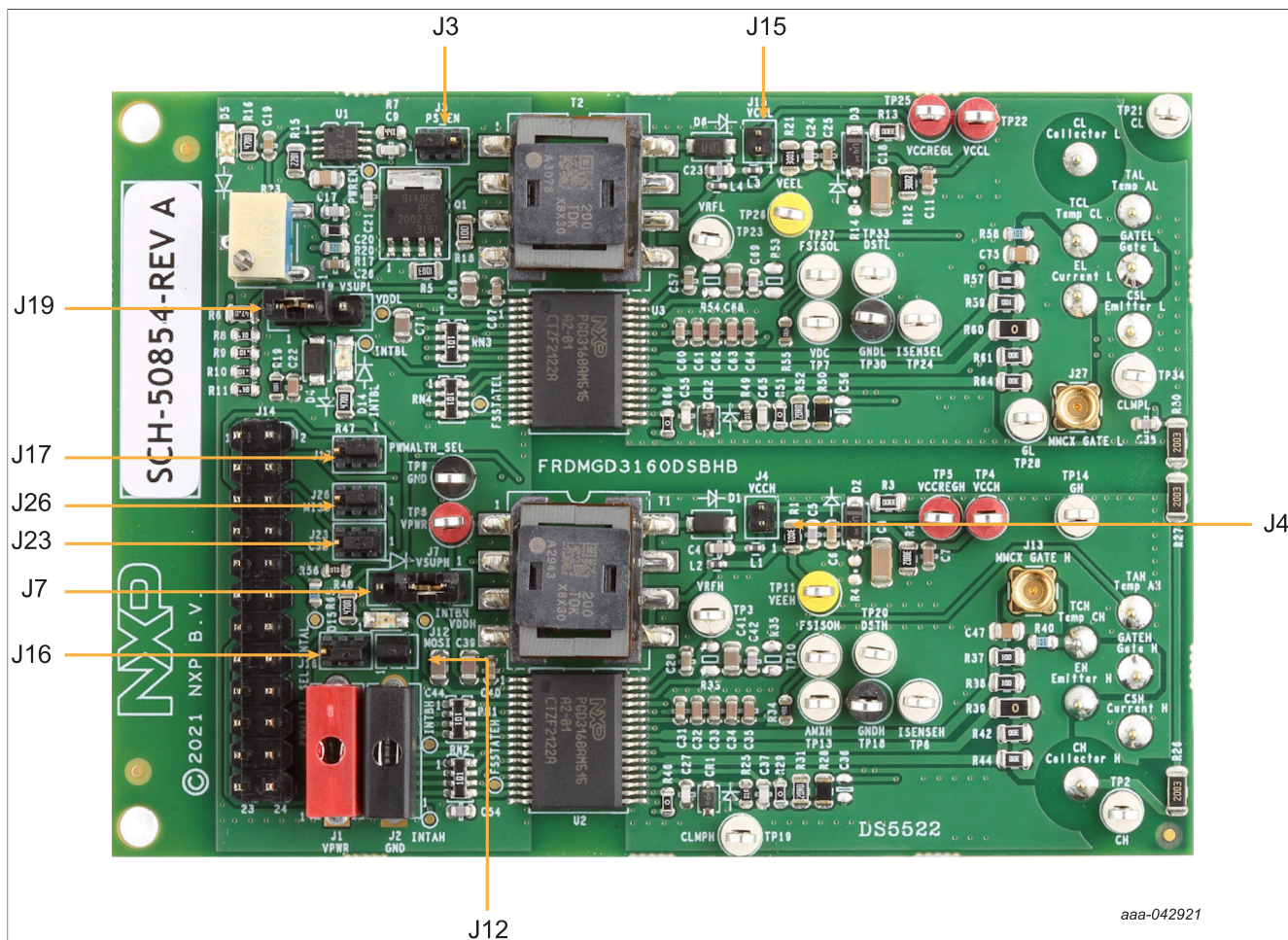
Figure 4. Power supply and jumper configuration
