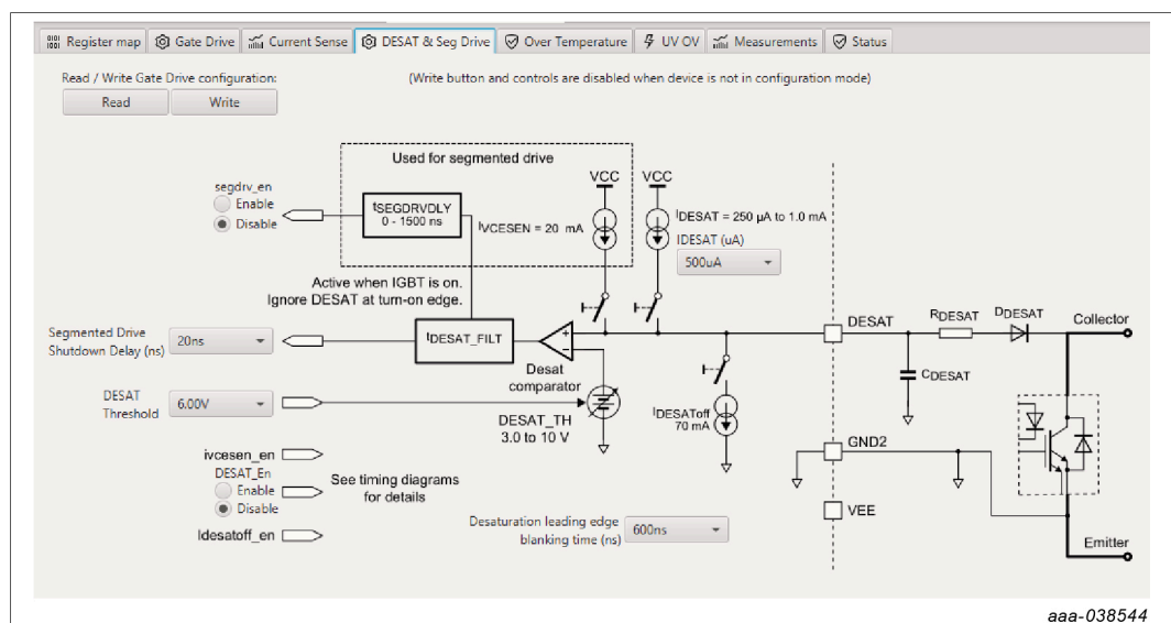
Figure 28. DESAT and Seg Drive tab
