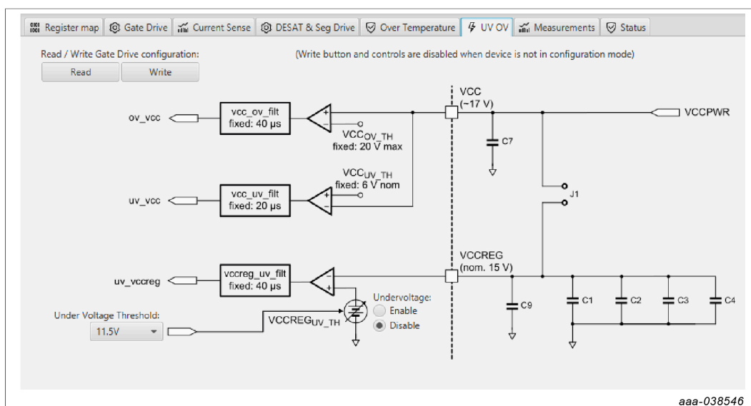
Figure 30. Undervoltage threshold tab
