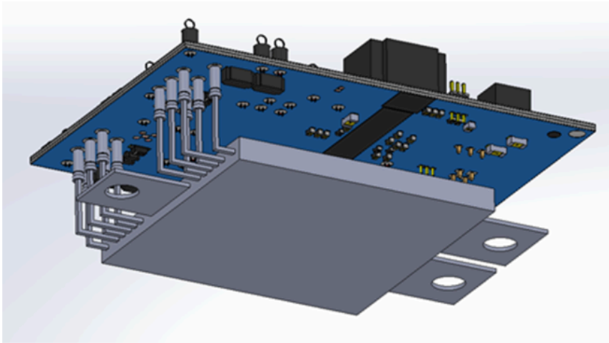
Figure 11. Evaluation board and power module connection
