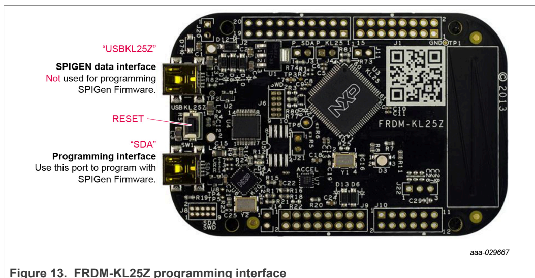
Figure 13. FRDM-KL25Z programming interface
