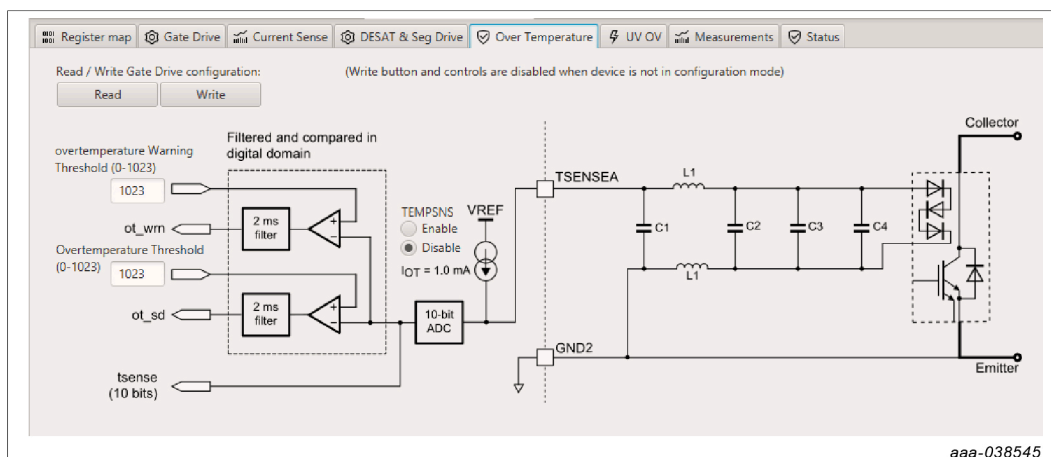
Figure 29. Over Temperature tab
