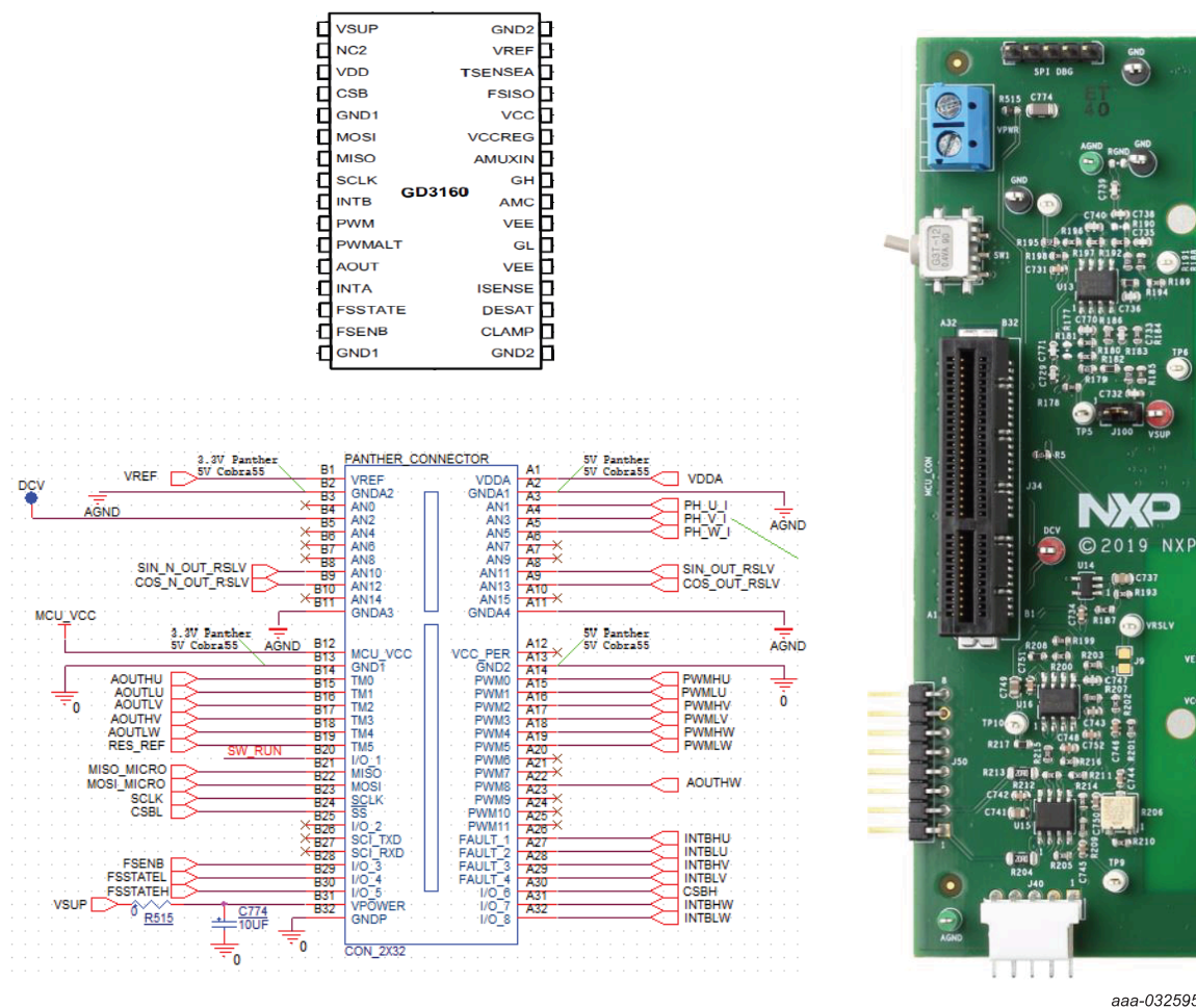
Figure 2. Gate driver pinout and board interface connection PCIe 2 x 32
