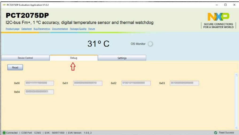
Figure 14. Graphical interface – “Debug” tab activated
