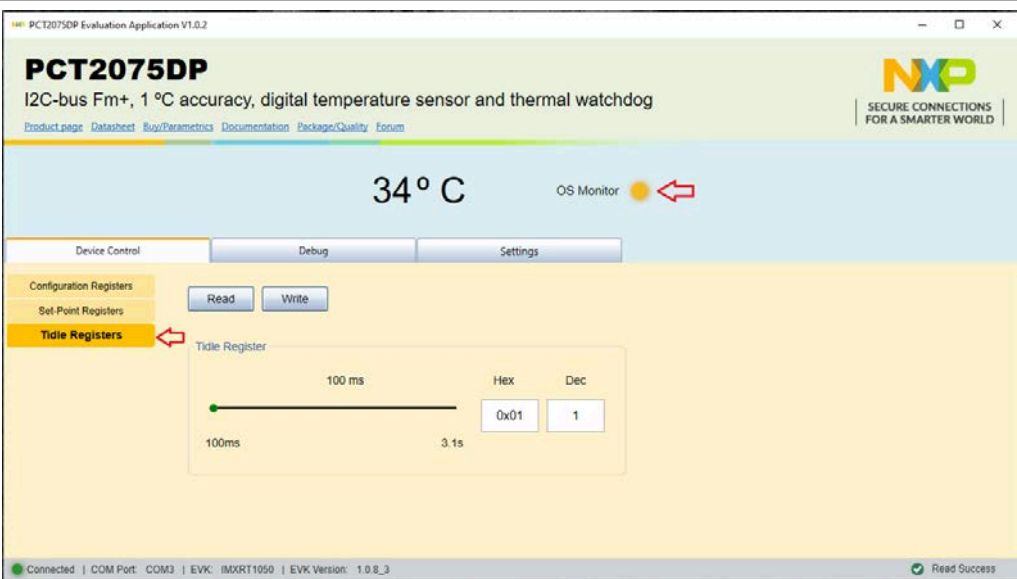
Figure 13. Graphical interface – “Device Control” / “Tidle Registers” tab activated
