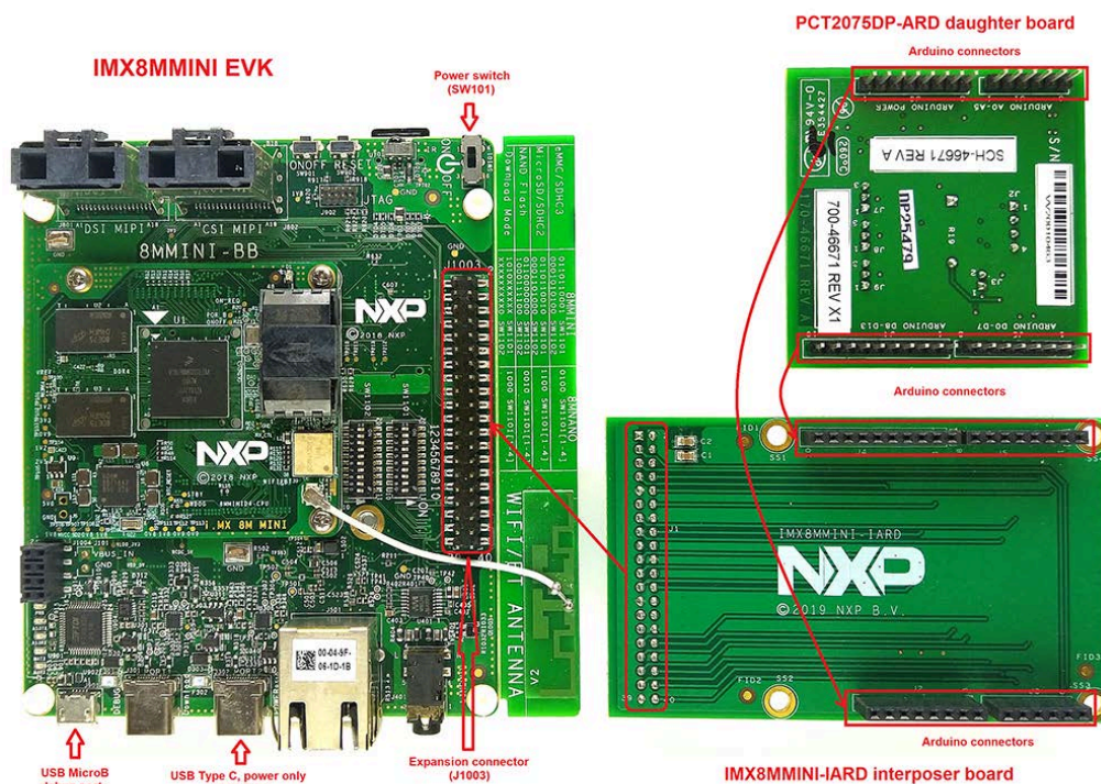
Figure 8. PCT2075DP-ARD daughterboard, IMX8MMINI-IARD interposer board, and 8MMINILPD4-EVK board assembly
