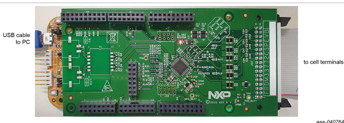
Figure 6. FRDM33772CSPEVB mounted to an S32K144EVB
