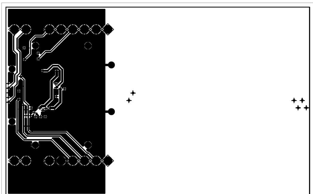
Figure 7. OM27160 board layer 3
