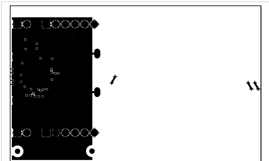
Figure 8. OM27160 board layer 4
