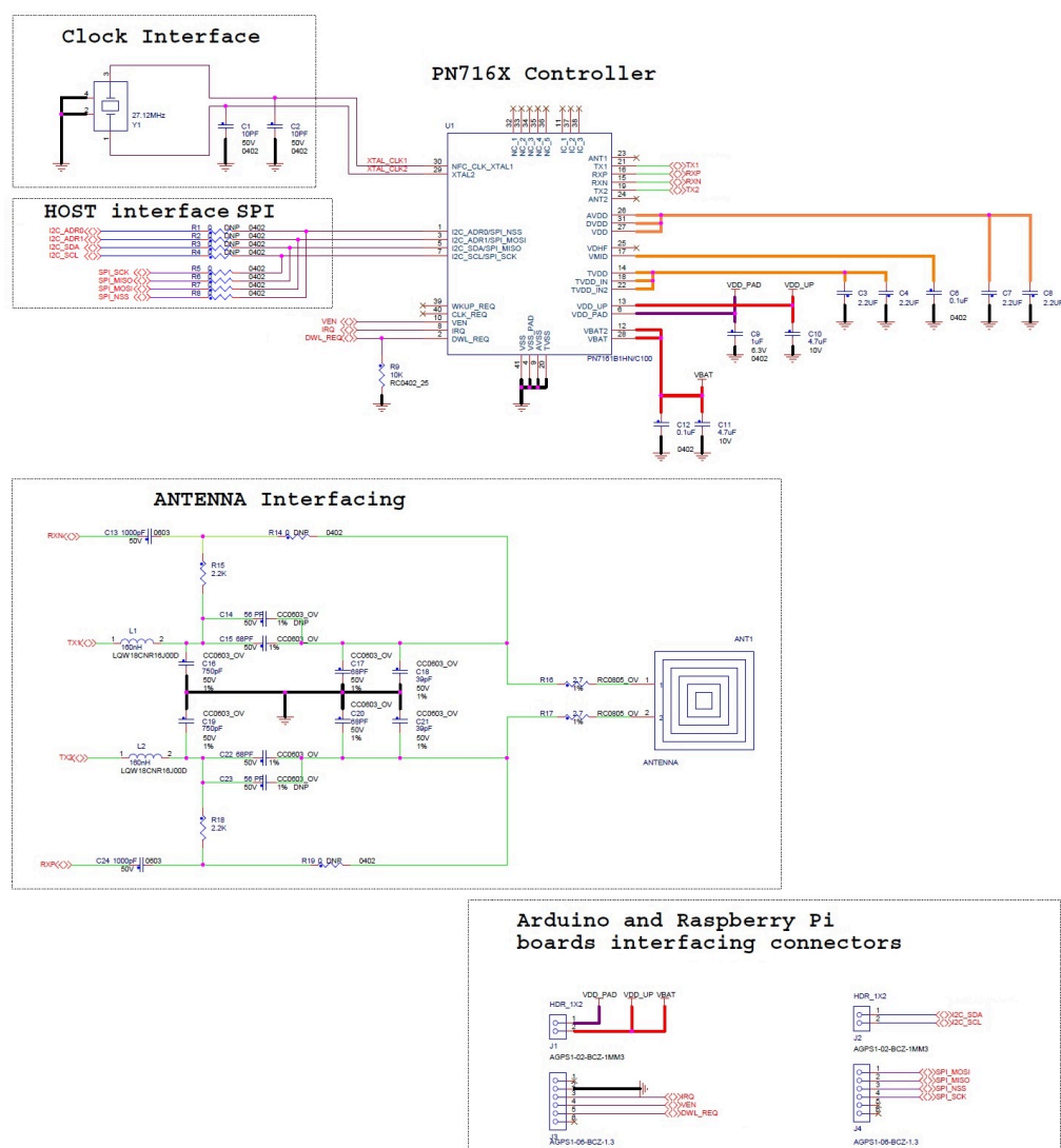
Figure 3. OM27160B1HN board schematics
