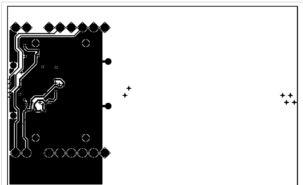
Figure 6. OM27160 board layer 2
