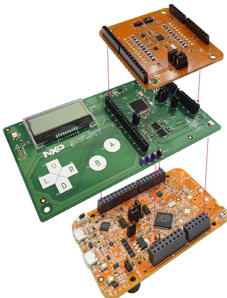
Figure 4. Physical connection
