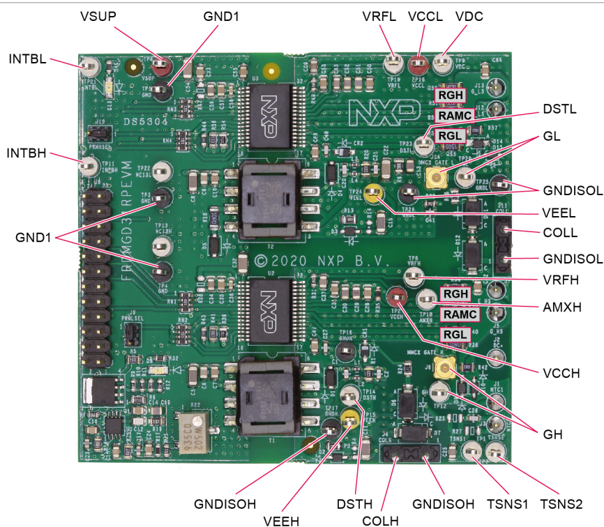
Figure 4. Key test point locations
