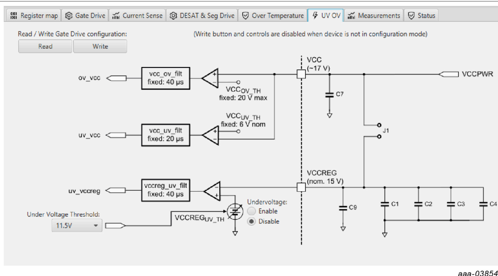
Figure 29. Undervoltage and overvoltage tab
