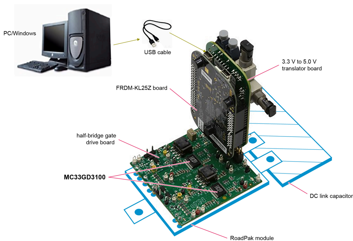
Figure 11. Evaluation board and system setup
