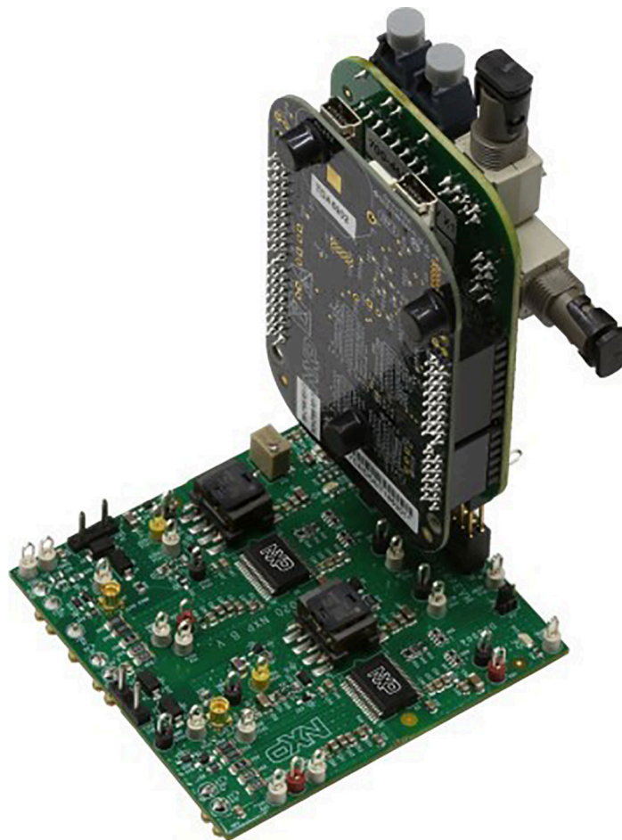
Figure 1. FRDMGD31RPEVM
