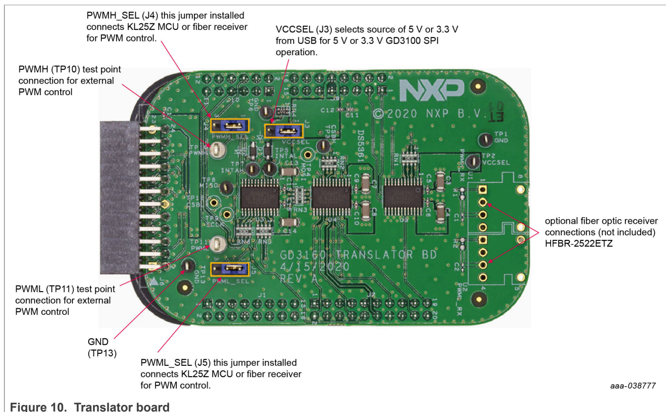
Figure 10. Translator board
