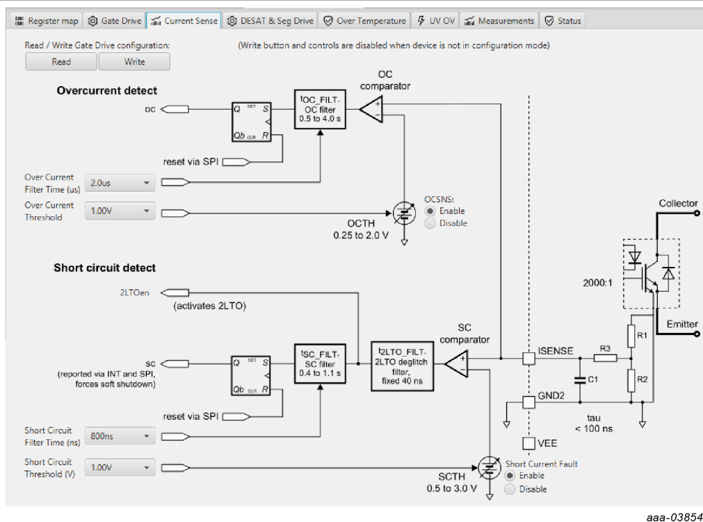
Figure 26. Current sense tab
