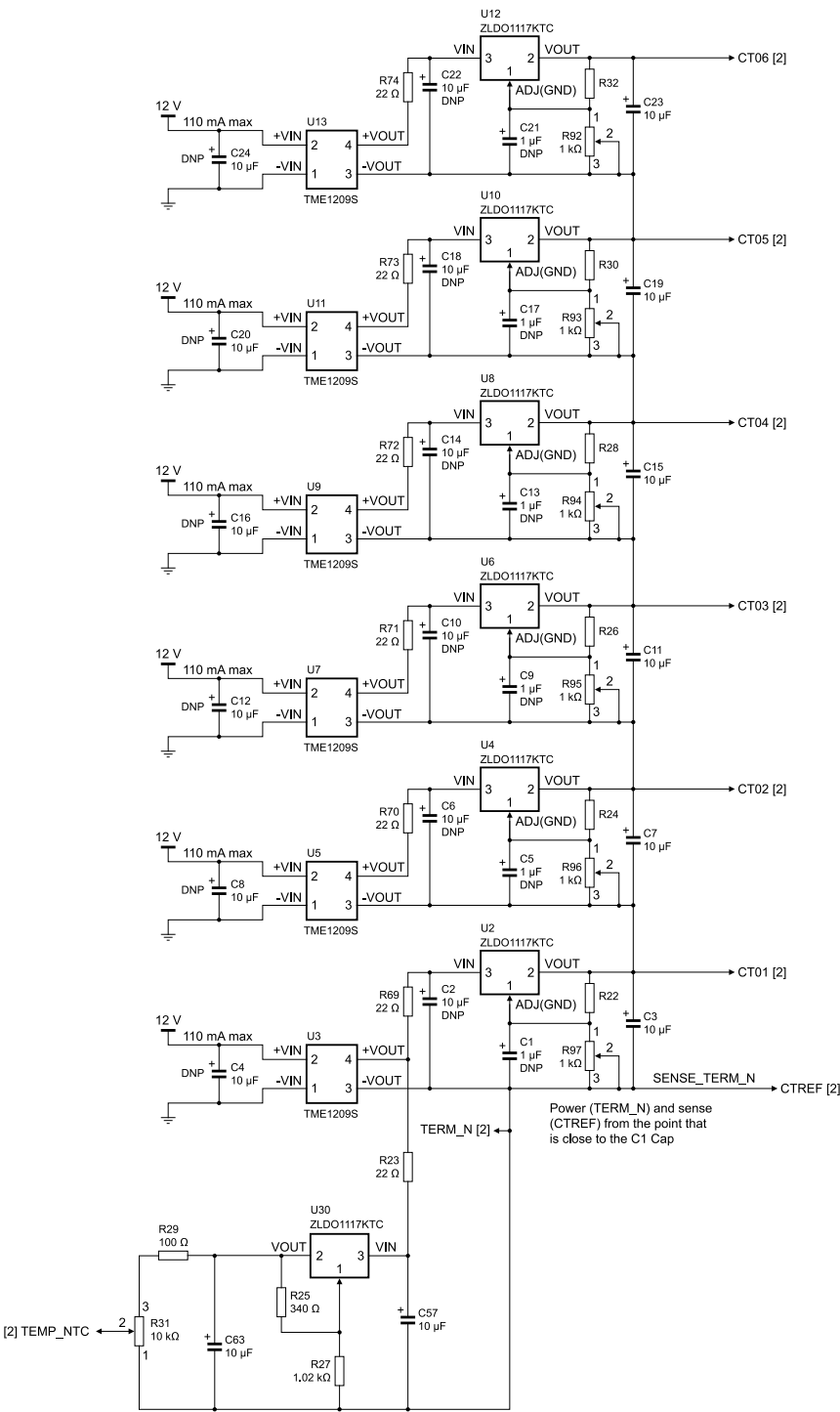
Figure 3. BATT-14CEMULATOR schematic (part 2)
