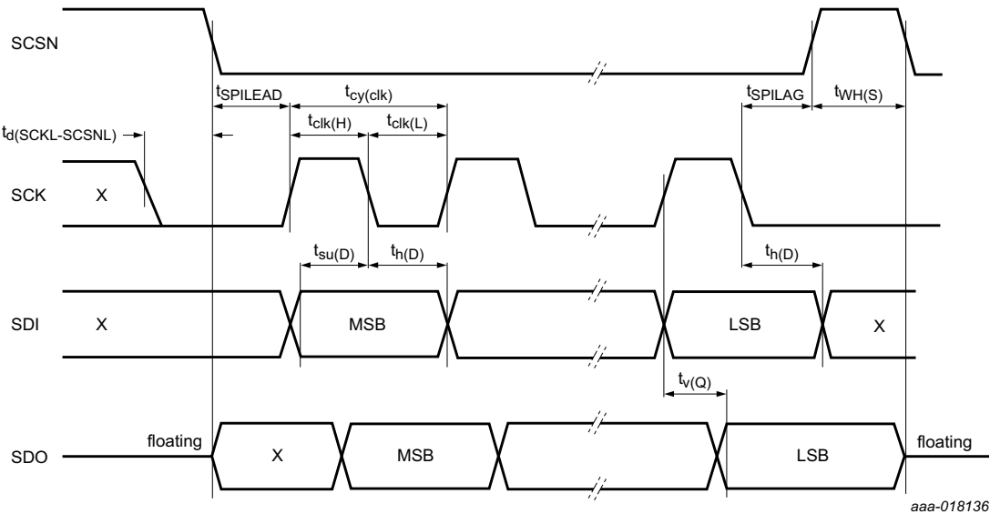
Fig 30. SPI timing diagram
