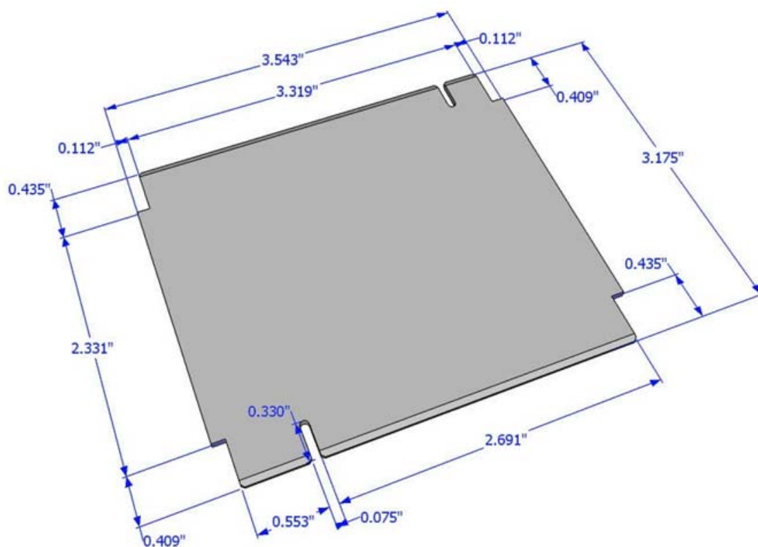
Figure 4. Board dimensions
