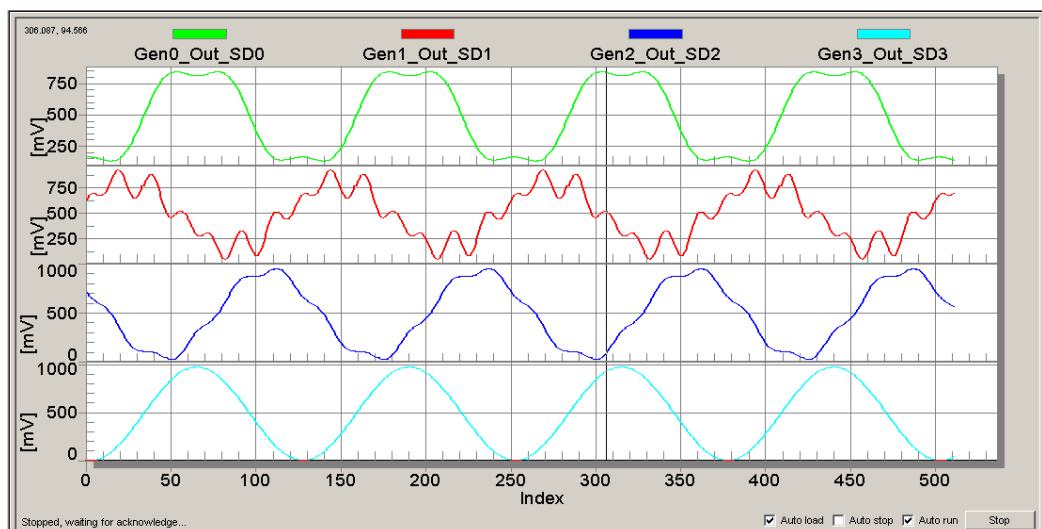
Figure 9. Example of generated harmonic signals in FreeMaster Recorder window
