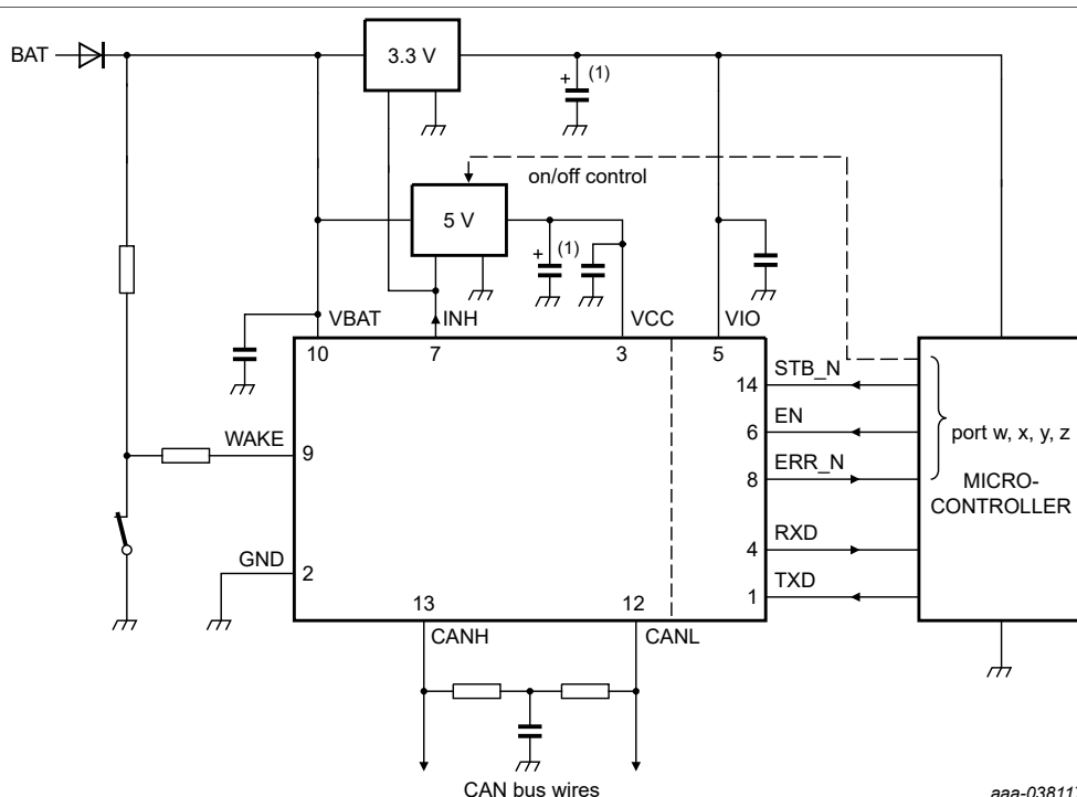
Figure 10. Typical TJR1443 application with a 3.3 V microcontroller
