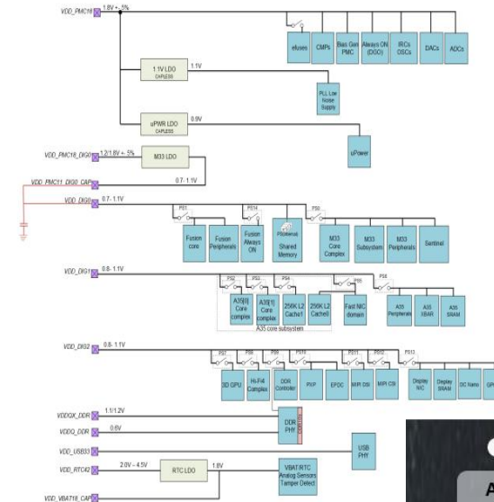
TOP LEVEL POWER CONTROL
