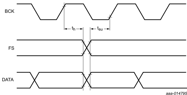
Fig 4. TDM/I 2 S timing
