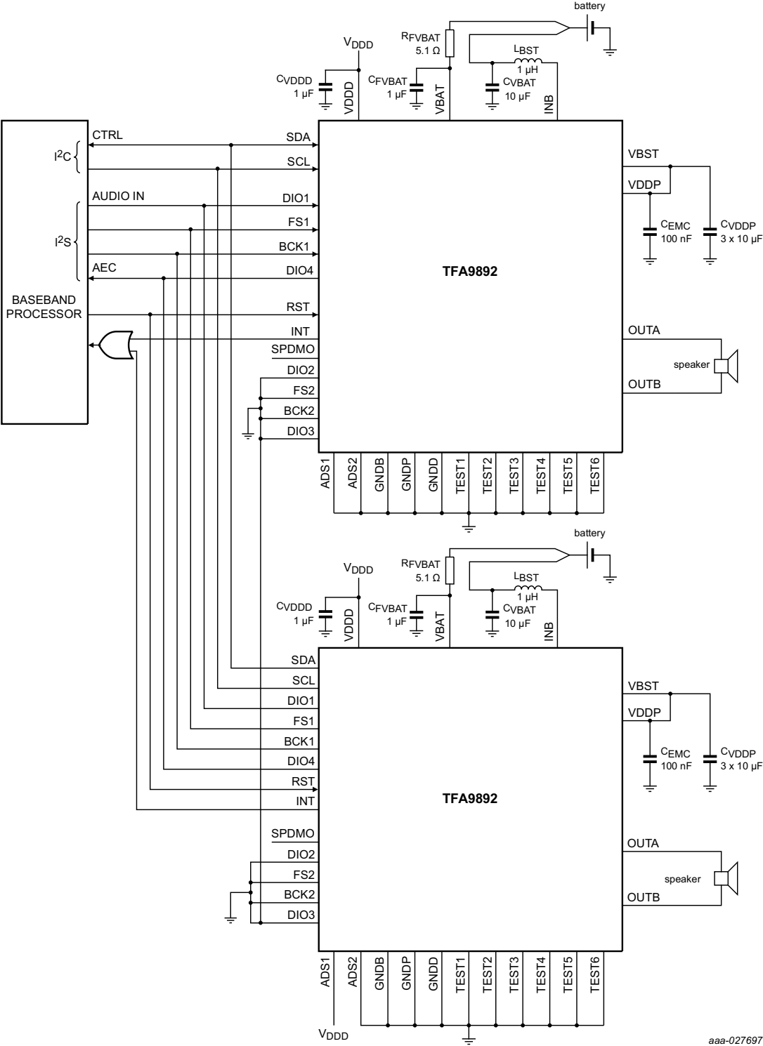
Fig 7. Typical stereo application
