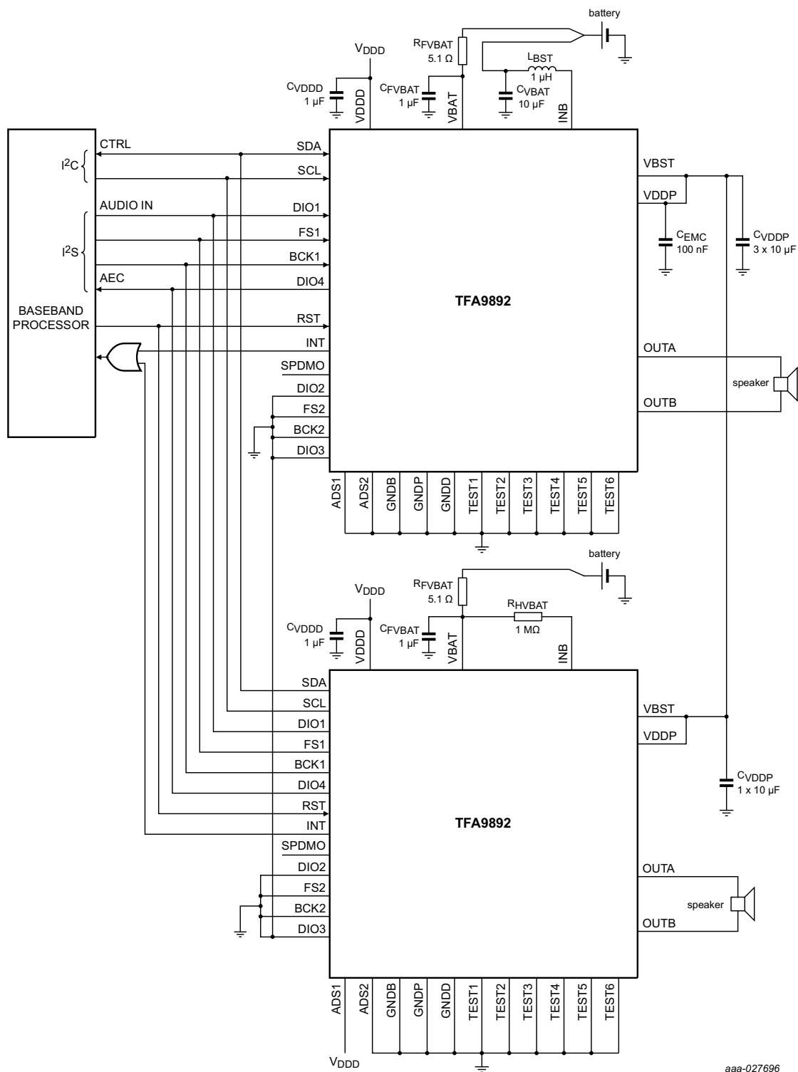
Fig 8. Stereo application using single coil
