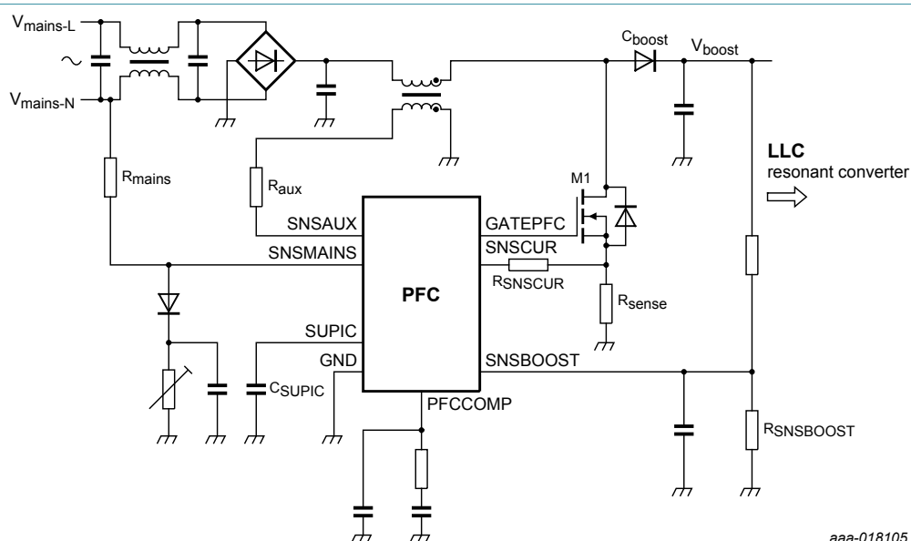
Figure 13. Application diagram
