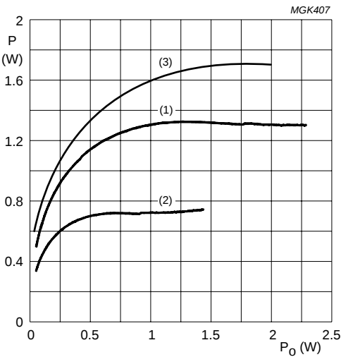
Sine wave of 1 kHz. (1) V_{CC} = 9\text{ V} , R_L = 16\ \Omega . (2) V_{CC} = 5\text{ V} , R_L = 8\ \Omega . (3) V_{CC} = 7.5\text{ V} , R_L = 8\ \Omega .
