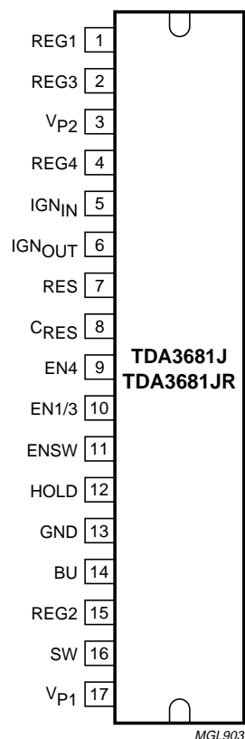
Fig.3 Pin configuration for TDA3681J and TDA3681JR.
