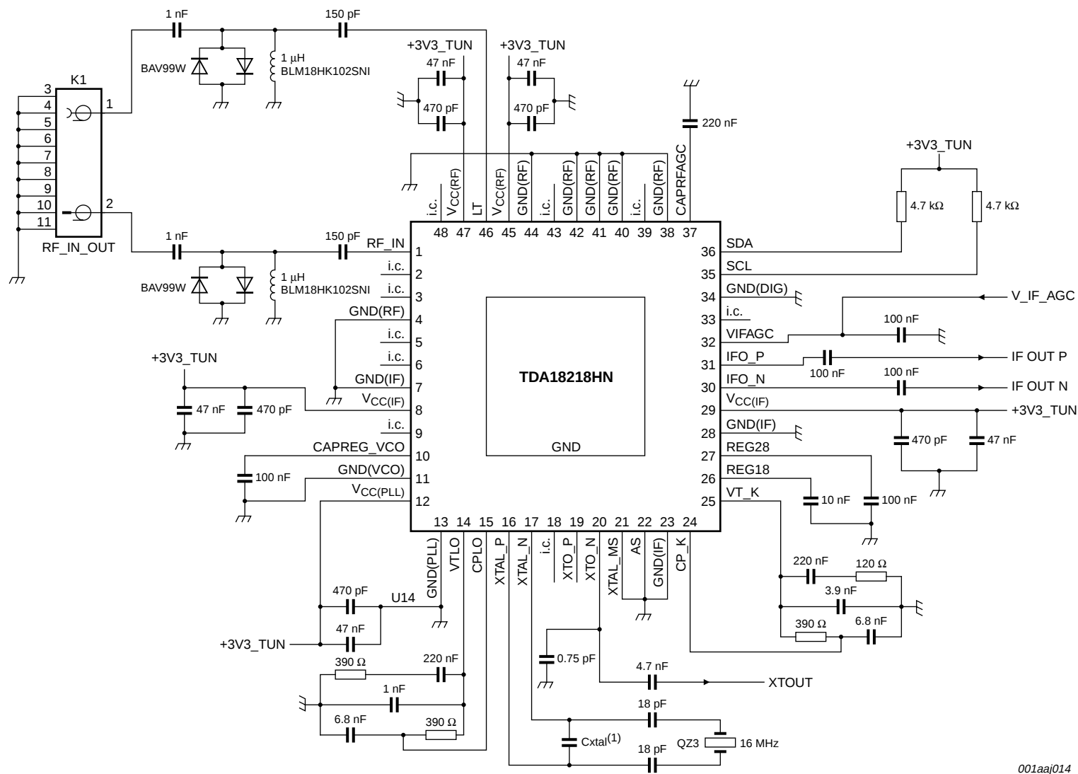
Fig 3. Application diagram
