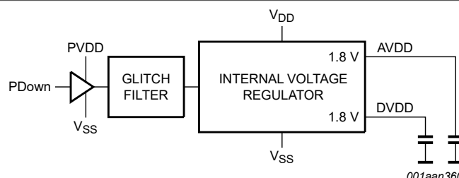
Figure 26. Internal PDown to voltage regulator logic
