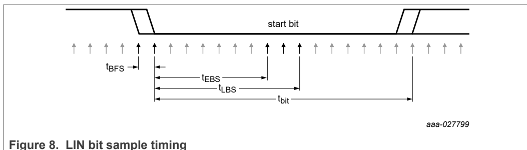
Figure 8. LIN bit sample timing
