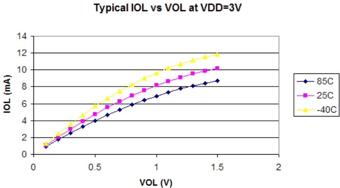
Figure 12-12. Typical I_{OL} vs. V_{OL} V_{DD} = 3\text{ V}
