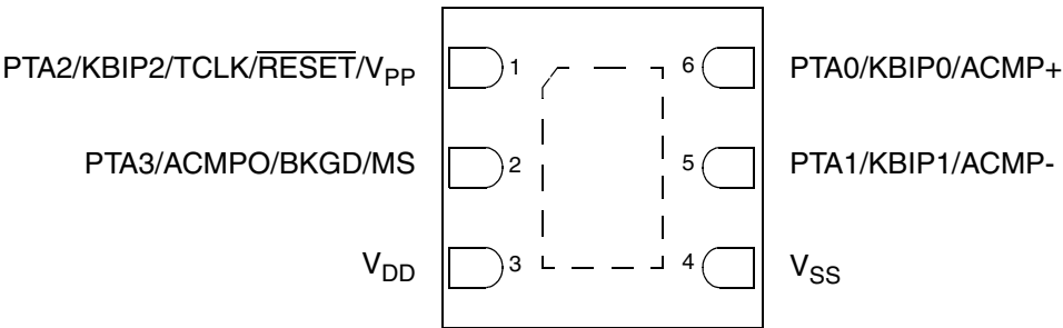
Figure 2-1. SC9RS08KA2 Series in 6-Pin DFN
