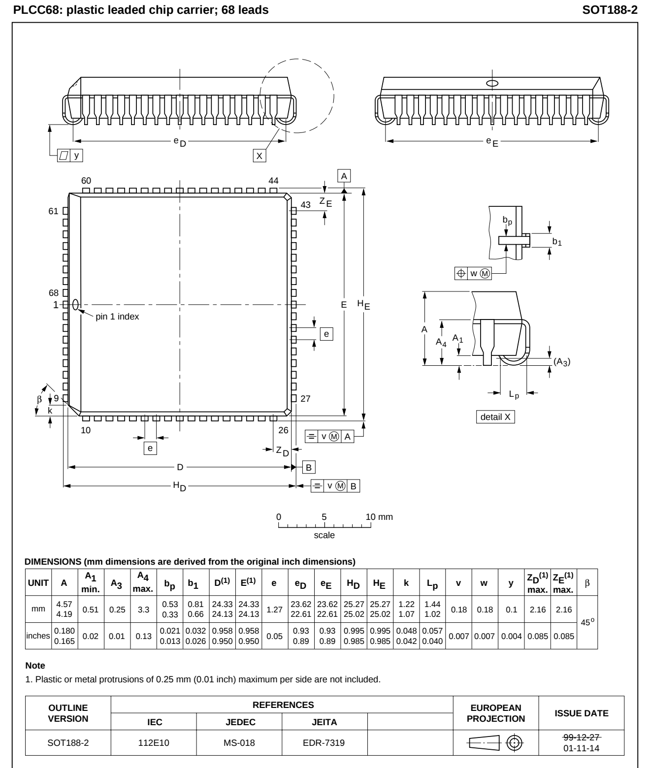
Fig 27. Package outline SOT188-2 (PLCC68)
