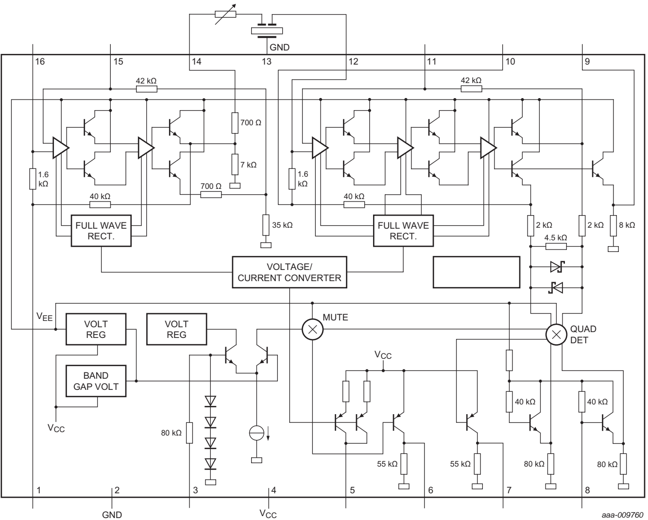
Fig 4. Equivalent circuit
