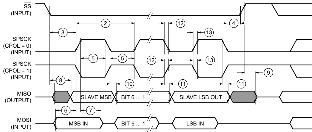
Figure 46. LPSPI Slave Mode Timing (CPHA=0)
