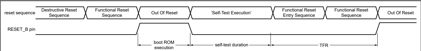
Figure 19. Start-up self-test
