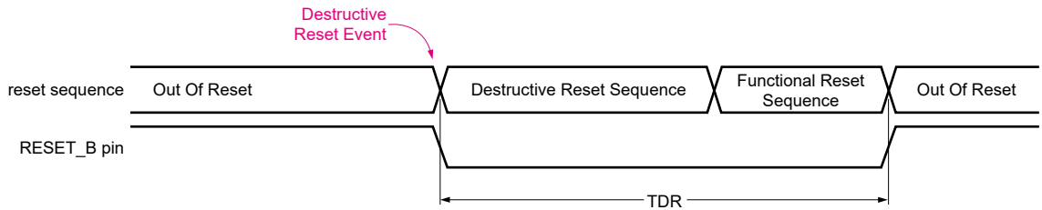
Figure 15. Destructive reset
