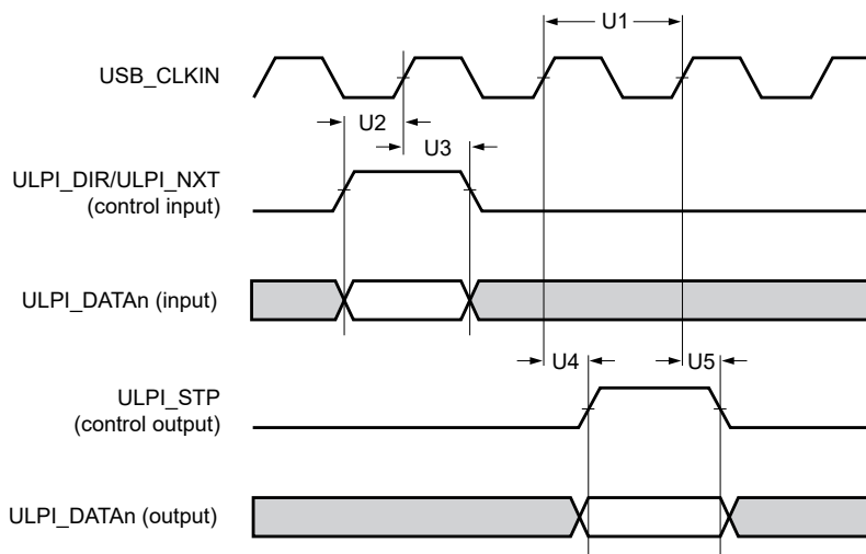
Figure 59. ULPI Mode Interface Timing
