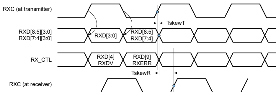
Figure 56. RGMII Receive Timing
