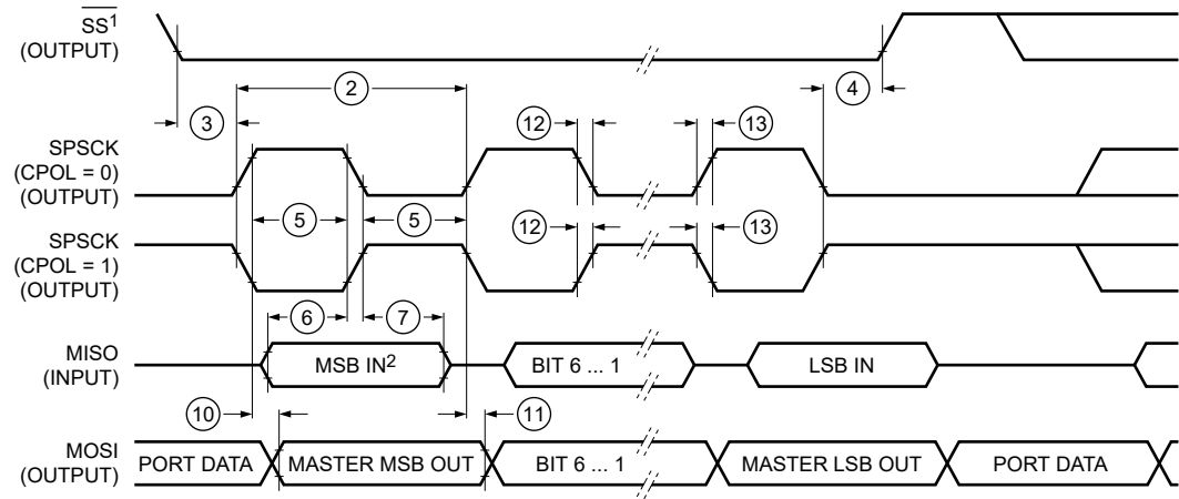
Figure 42. LPSPi Master Mode Timing (CPHA=1)
