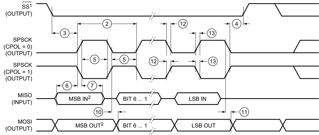
Figure 41. LPSPi Master Mode Timing (CPHA=0)
