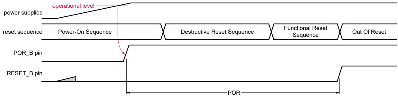
Figure 18. Initial power-up
