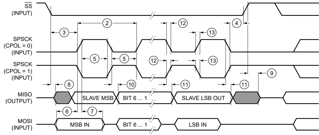
Figure 43. LPSPi Slave Mode Timing (CPHA=0)
