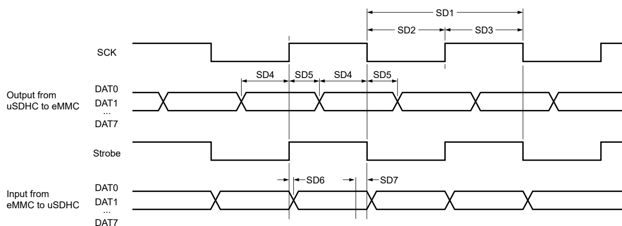
Figure 71. HS400 Mode Interface Timing
