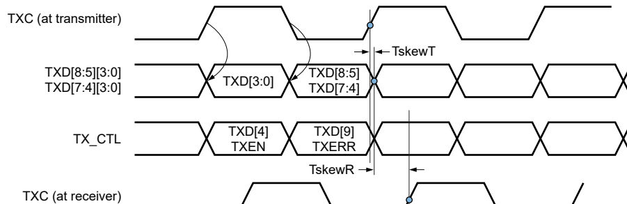
Figure 57. RGMII Transmit Timing
