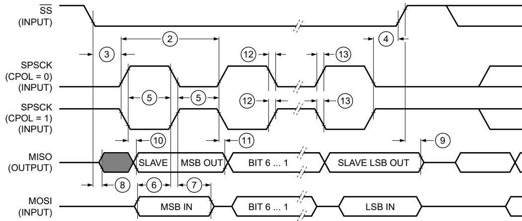
Figure 44. LPSPi Slave Mode Timing (CPHA=1)
