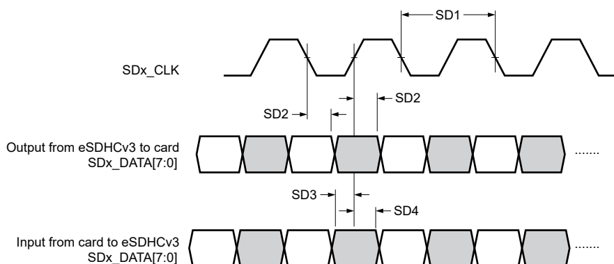
Figure 67. SD3.0/eMMC5.1 DDR Mode Interface Timing
