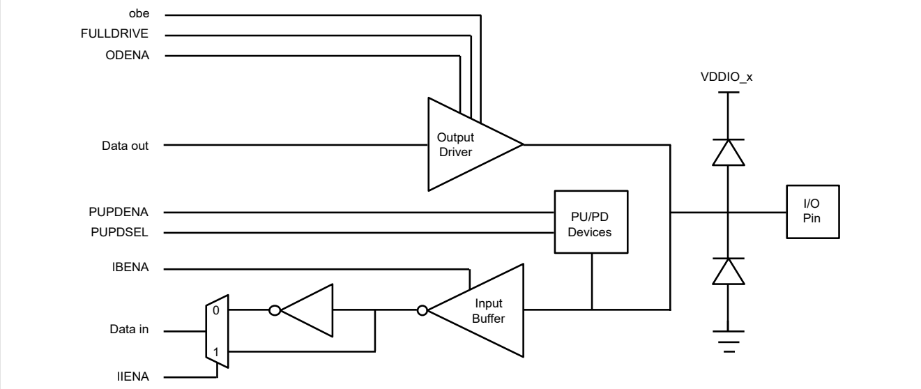
Figure 33. Simplified high-speed GPIO pins
