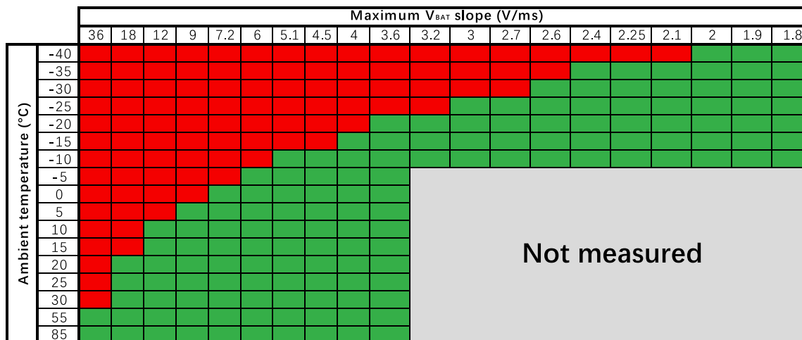
Fig 11. Maximum V_{BAT} slope vs temperature
