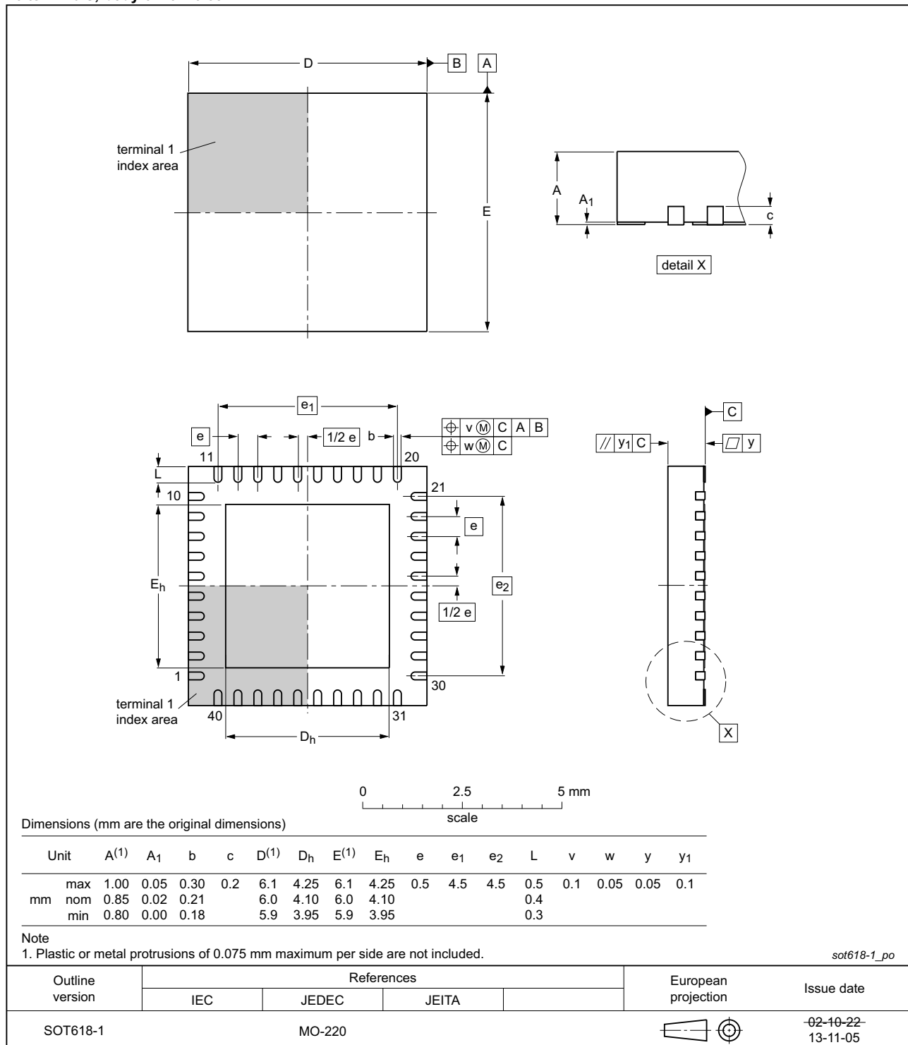
Fig 20. Package outline SOT618-1 HVQFN40
