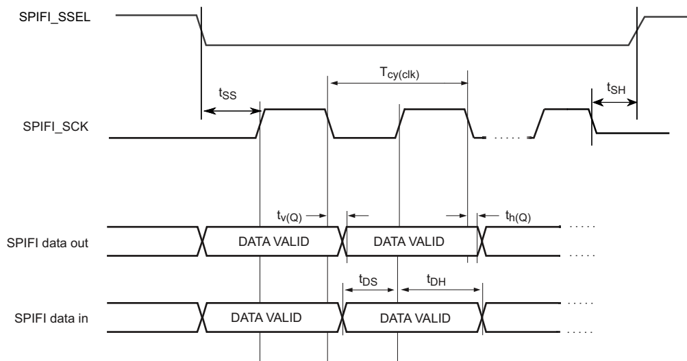
Fig 17. SPIFI interface timings
