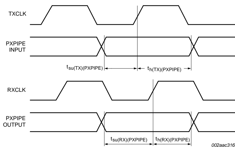
Fig 18. Definition of PXPIPE timing
