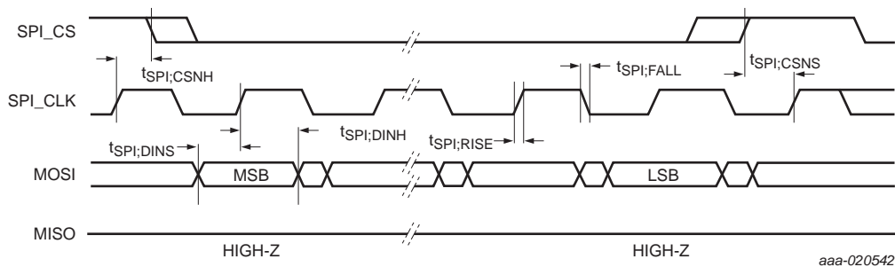
Fig 9. SPI write timing
