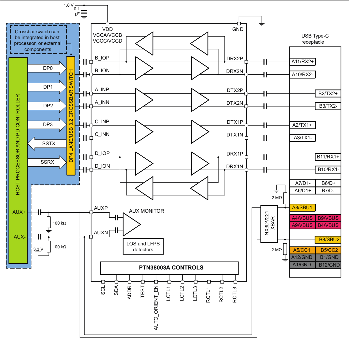
Figure 3. Connection illustration when PTN38003A in DFP receptacle application
