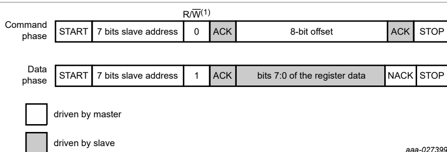
Figure 9. I 2 C read sequence
