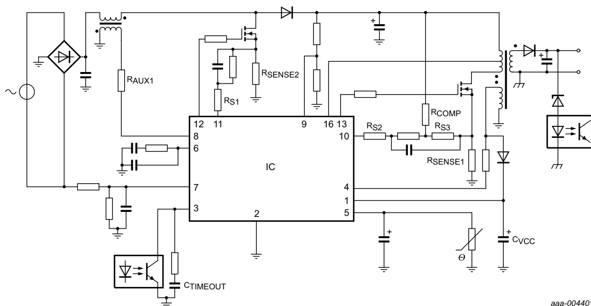
Fig 17. Typical application diagram for the TEA1752T IC
