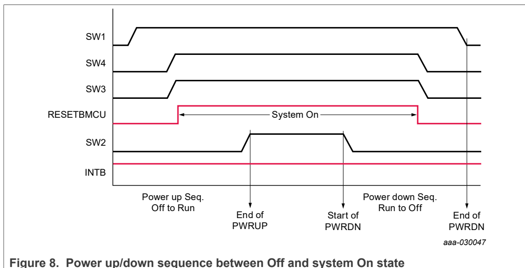
Figure 8. Power up/down sequence between Off and system On state
