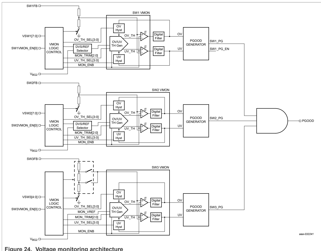
Figure 24. Voltage monitoring architecture
